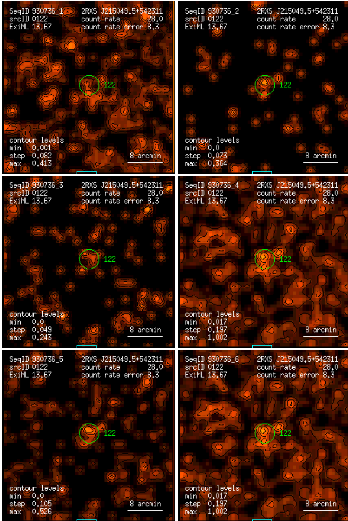
Figure 122: RASS 930736: detection 0122: band rate images, Gaussian filter: (1) PSPC channels 11 – 41, (2) 52 – 90, (3) 91 – 201, (4) 11 – 235, (5) 52 – 201, (6) 11 – 201. Broad band rates in counts/ks. Band rate contour levels in counts/ks/arcmin 2 .
