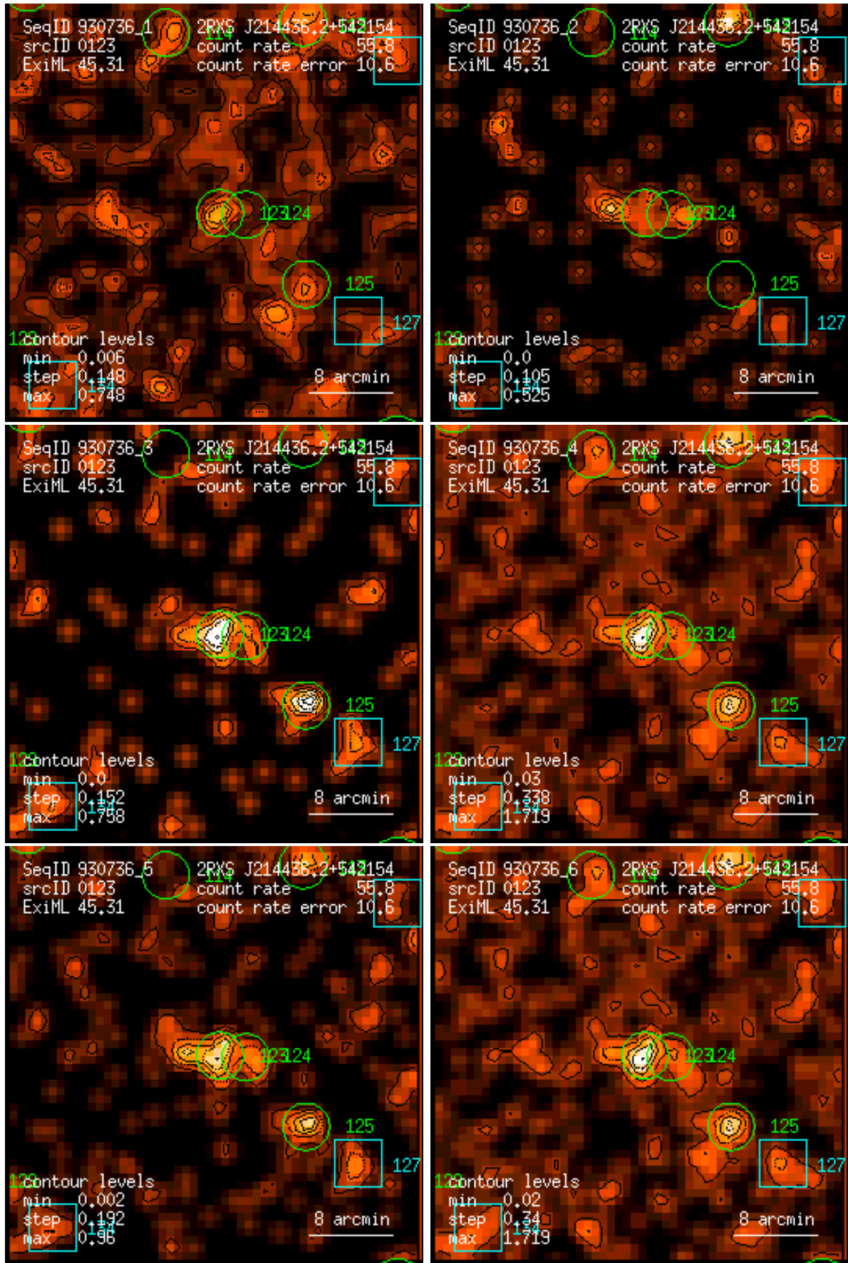
Figure 123: RASS 930736: detection 0123: band rate images, Gaussian filter: (1) PSPC channels 11 – 41, (2) 52 – 90, (3) 91 – 201, (4) 11 – 235, (5) 52 – 201, (6) 11 – 201. Broad band rates in counts/ks. Band rate contour levels in counts/ks/arcmin 2 .
