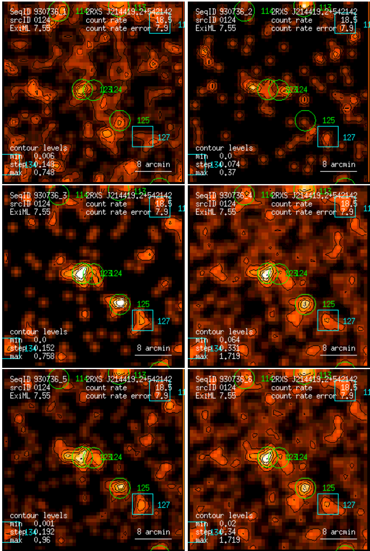
Figure 124: RASS 930736: detection 0124: band rate images, Gaussian filter: (1) PSPC channels 11 – 41, (2) 52 – 90, (3) 91 – 201, (4) 11 – 235, (5) 52 – 201, (6) 11 – 201. Broad band rates in counts/ks. Band rate contour levels in counts/ks/arcmin 2 .
