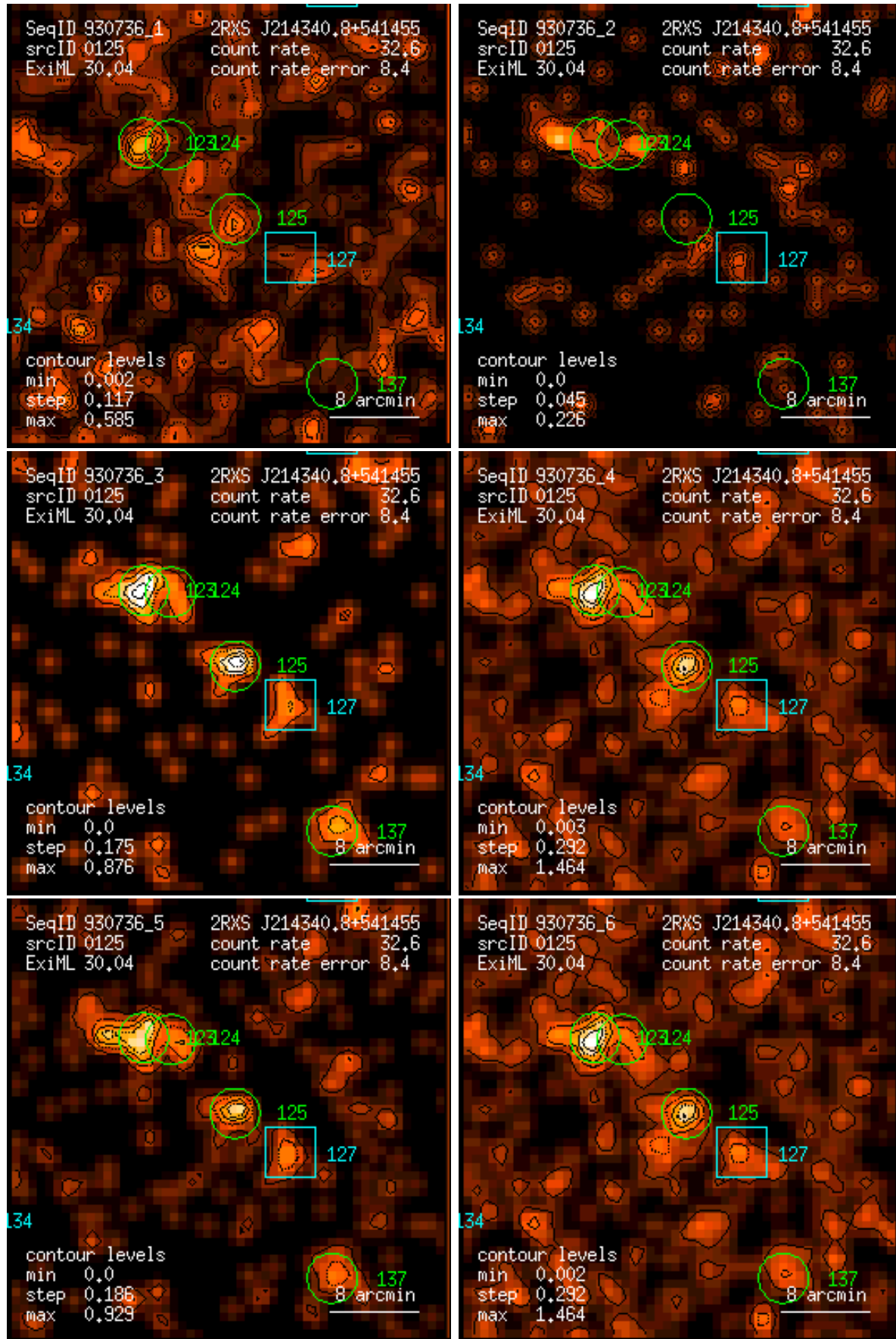
Figure 125: RASS 930736: detection 0125: band rate images, Gaussian filter: (1) PSPC channels 11 – 41, (2) 52 – 90, (3) 91 – 201, (4) 11 – 235, (5) 52 – 201, (6) 11 – 201. Broad band rates in counts/ks. Band rate contour levels in counts/ks/arcmin 2 .
