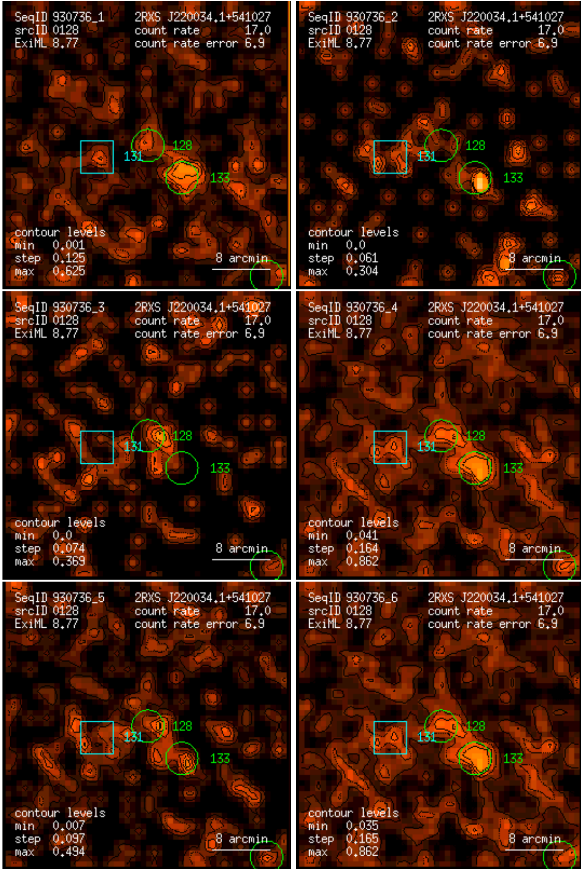
Figure 128: RASS 930736: detection 0128: band rate images, Gaussian filter: (1) PSPC channels 11 – 41, (2) 52 – 90, (3) 91 – 201, (4) 11 – 235, (5) 52 – 201, (6) 11 – 201. Broad band rates in counts/ks. Band rate contour levels in counts/ks/arcmin 2 .
