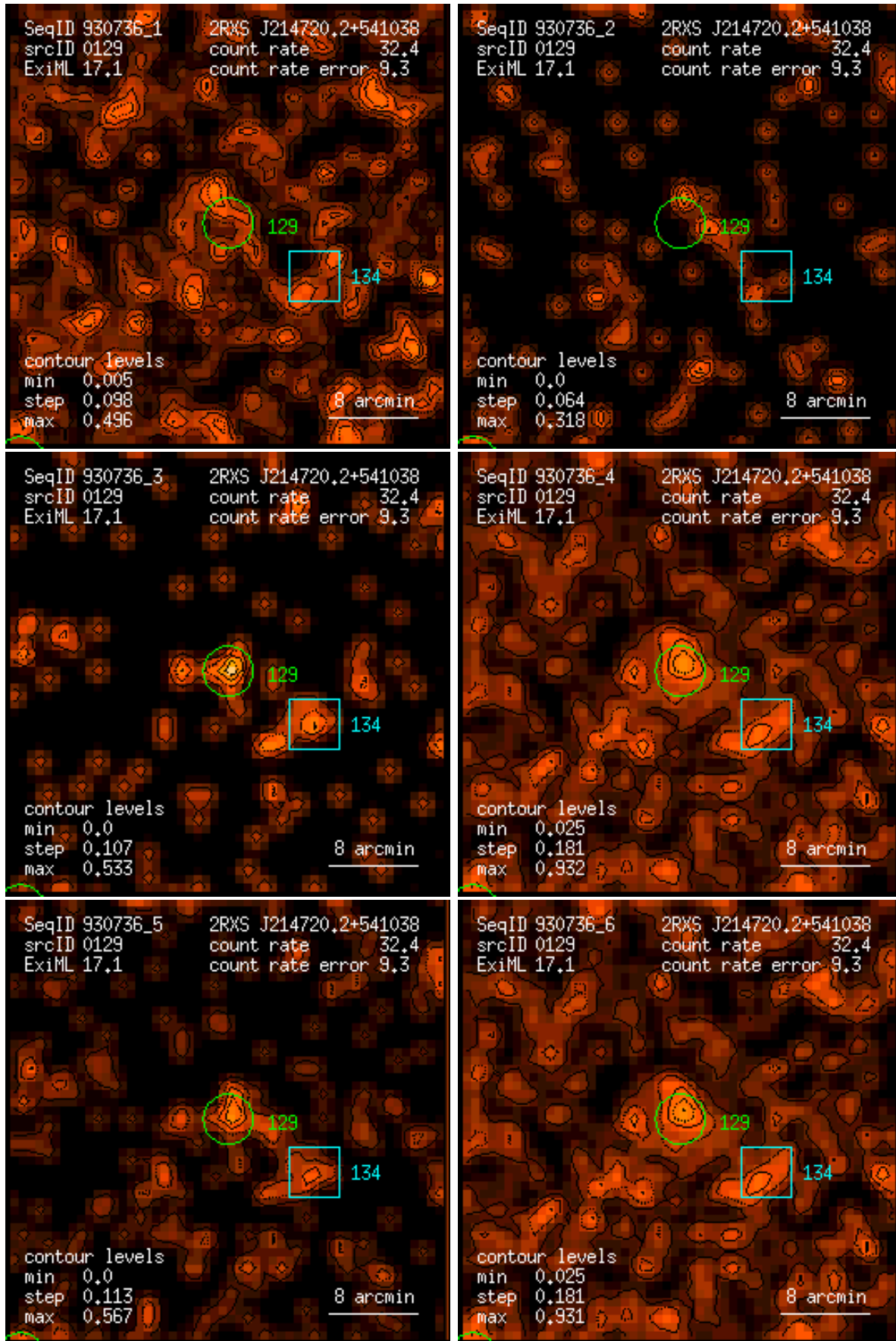
Figure 129: RASS 930736: detection 0129: band rate images, Gaussian filter: (1) PSPC channels 11 – 41, (2) 52 – 90, (3) 91 – 201, (4) 11 – 235, (5) 52 – 201, (6) 11 – 201. Broad band rates in counts/ks. Band rate contour levels in counts/ks/arcmin 2 .
