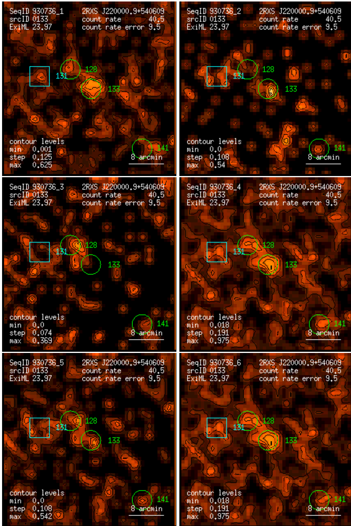
Figure 133: RASS 930736: detection 0133: band rate images, Gaussian filter: (1) PSPC channels 11 – 41, (2) 52 – 90, (3) 91 – 201, (4) 11 – 235, (5) 52 – 201, (6) 11 – 201. Broad band rates in counts/ks. Band rate contour levels in counts/ks/arcmin 2 .
