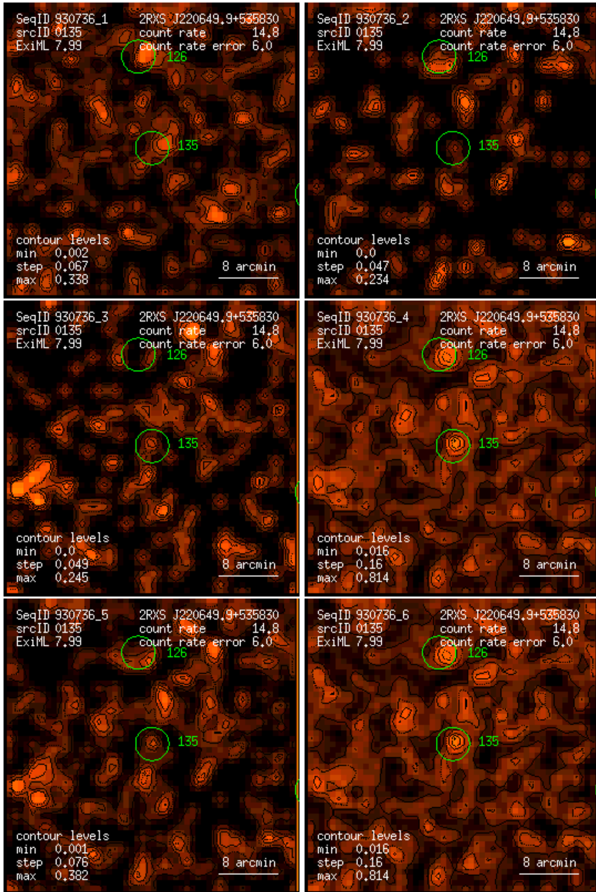
Figure 135: RASS 930736: detection 0135: band rate images, Gaussian filter: (1) PSPC channels 11 – 41, (2) 52 – 90, (3) 91 – 201, (4) 11 – 235, (5) 52 – 201, (6) 11 – 201. Broad band rates in counts/ks. Band rate contour levels in counts/ks/arcmin 2 .
