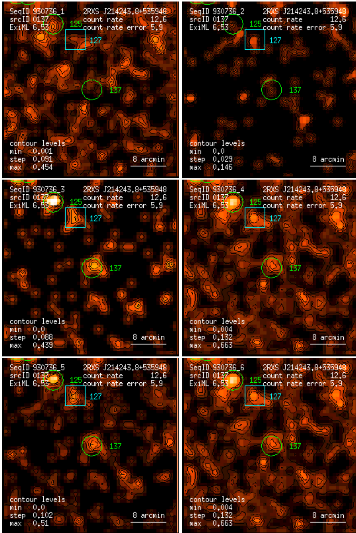
Figure 137: RASS 930736: detection 0137: band rate images, Gaussian filter: (1) PSPC channels 11 – 41, (2) 52 – 90, (3) 91 – 201, (4) 11 – 235, (5) 52 – 201, (6) 11 – 201. Broad band rates in counts/ks. Band rate contour levels in counts/ks/arcmin 2 .
