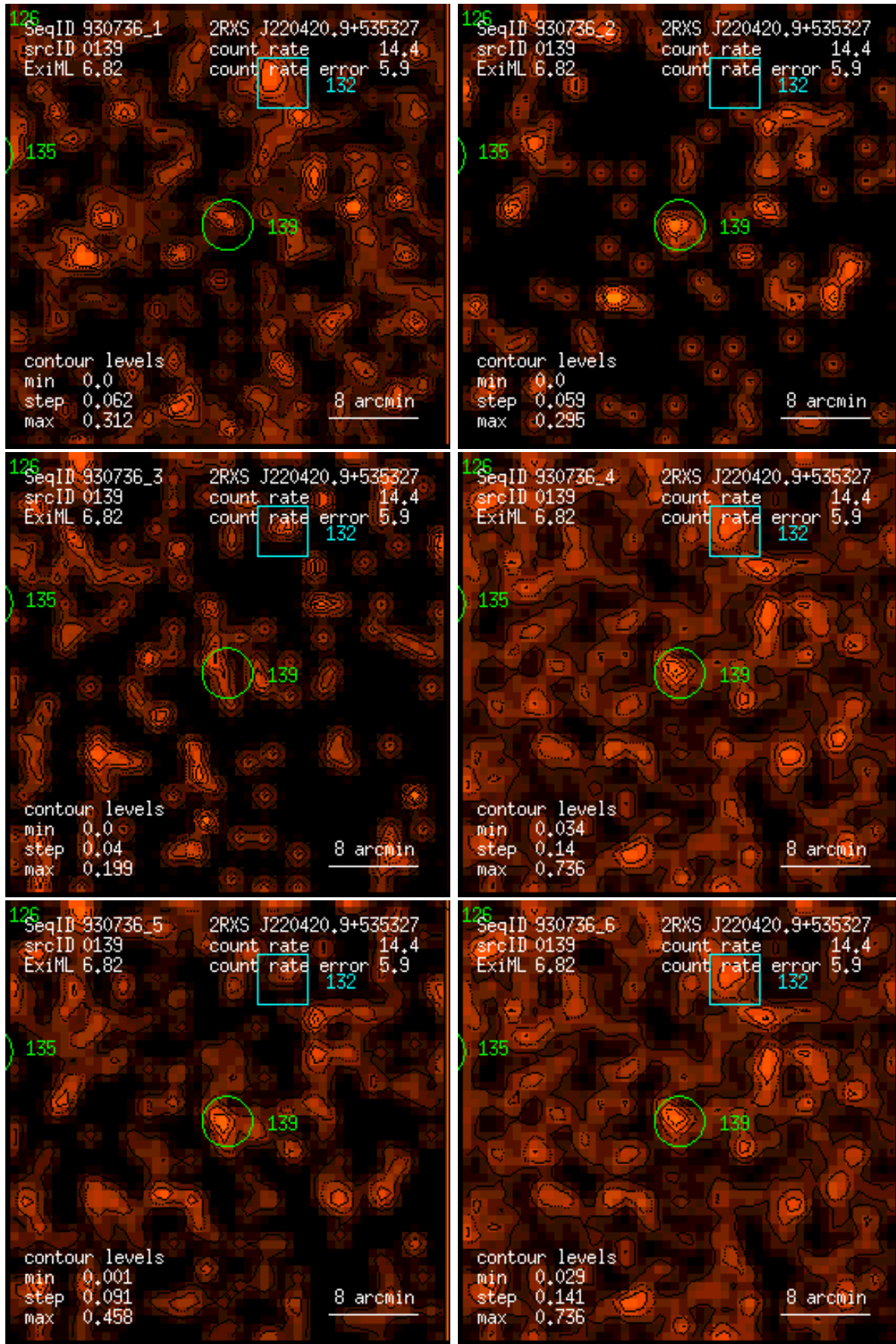
Figure 139: RASS 930736: detection 0139: band rate images, Gaussian filter: (1) PSPC channels 11 – 41, (2) 52 – 90, (3) 91 – 201, (4) 11 – 235, (5) 52 – 201, (6) 11 – 201. Broad band rates in counts/ks. Band rate contour levels in counts/ks/arcmin 2 .
