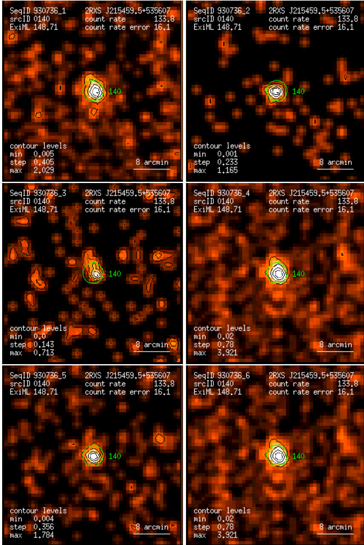
Figure 140: RASS 930736: detection 0140: band rate images, Gaussian filter: (1) PSPC channels 11 – 41, (2) 52 – 90, (3) 91 – 201, (4) 11 – 235, (5) 52 – 201, (6) 11 – 201. Broad band rates in counts/ks. Band rate contour levels in counts/ks/arcmin 2 .
