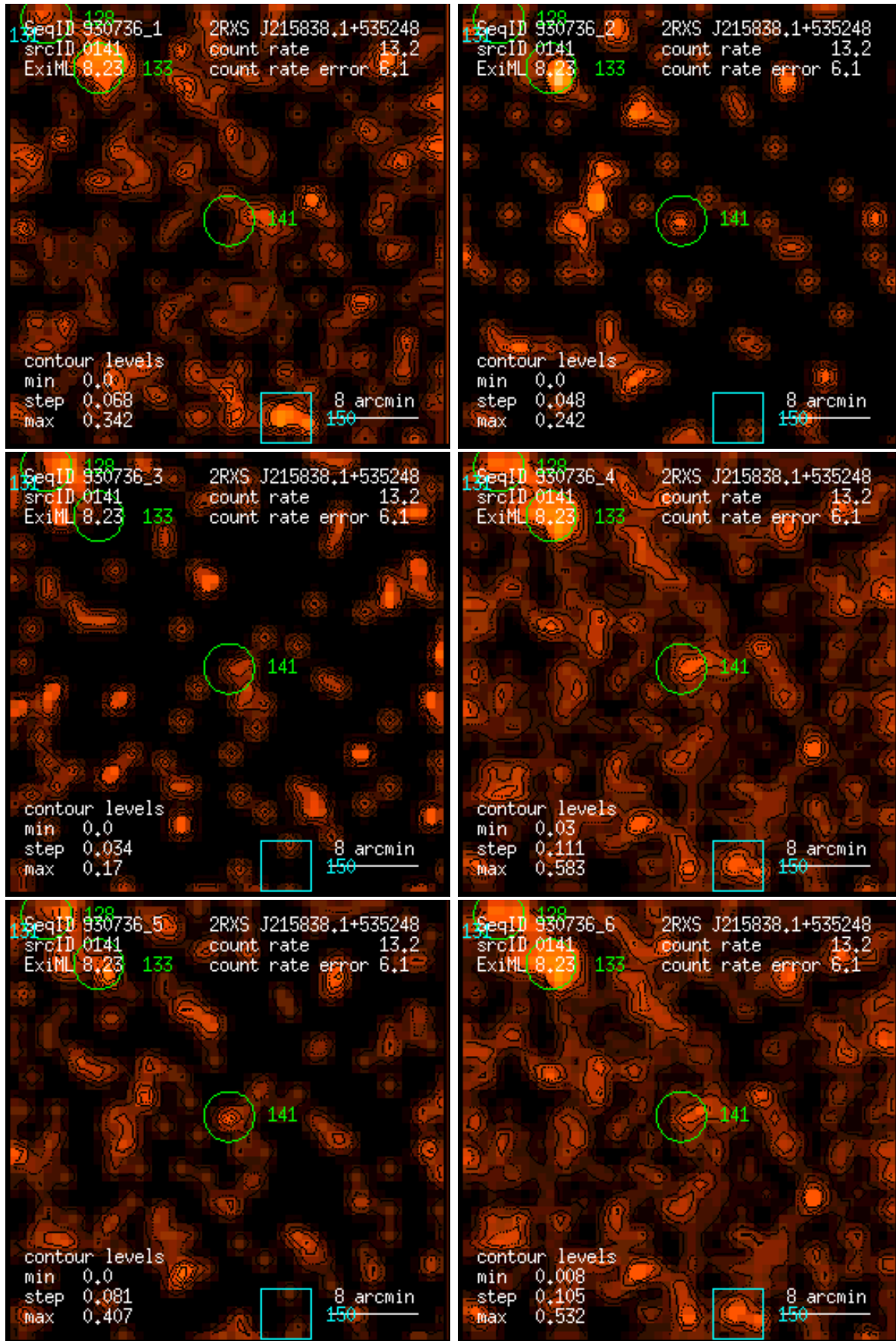
Figure 141: RASS 930736: detection 0141: band rate images, Gaussian filter: (1) PSPC channels 11 – 41, (2) 52 – 90, (3) 91 – 201, (4) 11 – 235, (5) 52 – 201, (6) 11 – 201. Broad band rates in counts/ks. Band rate contour levels in counts/ks/arcmin 2 .
