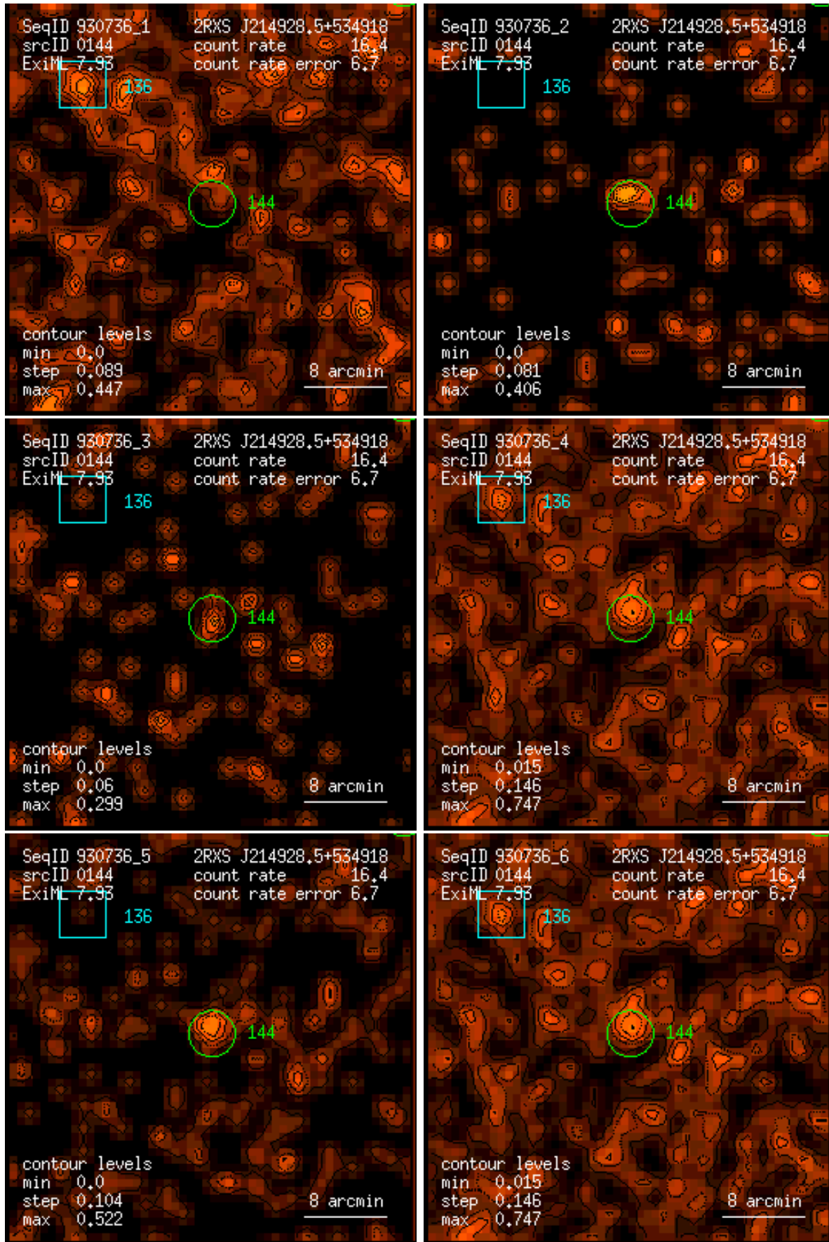
Figure 144: RASS 930736: detection 0144: band rate images, Gaussian filter: (1) PSPC channels 11 – 41, (2) 52 – 90, (3) 91 – 201, (4) 11 – 235, (5) 52 – 201, (6) 11 – 201. Broad band rates in counts/ks. Band rate contour levels in counts/ks/arcmin 2 .
