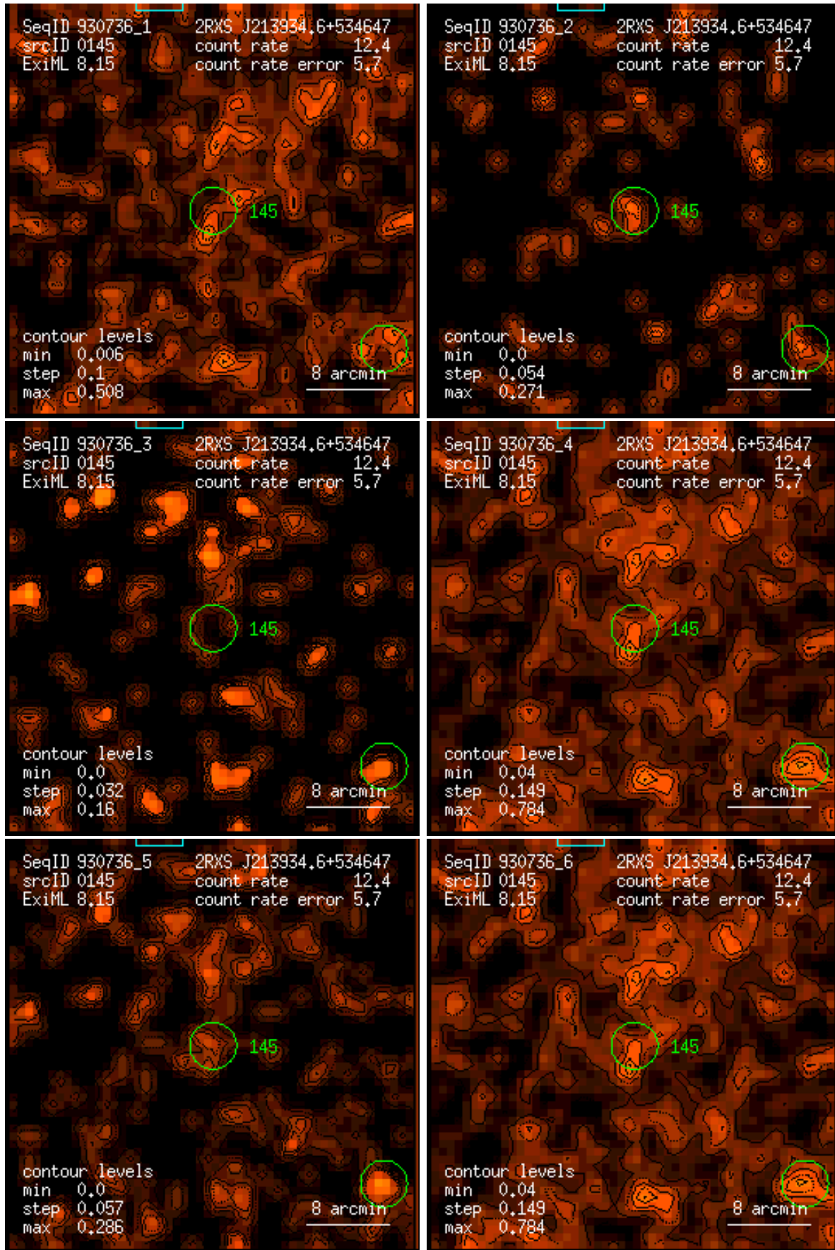
Figure 145: RASS 930736: detection 0145: band rate images, Gaussian filter: (1) PSPC channels 11 – 41, (2) 52 – 90, (3) 91 – 201, (4) 11 – 235, (5) 52 – 201, (6) 11 – 201. Broad band rates in counts/ks. Band rate contour levels in counts/ks/arcmin 2 .
