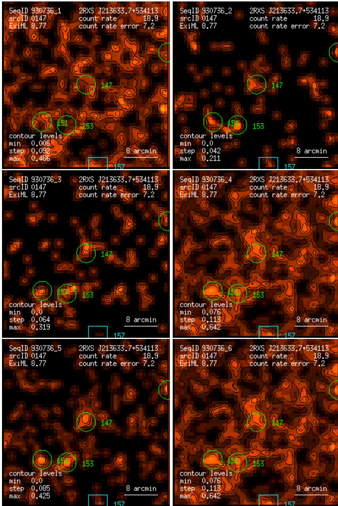
Figure 147: RASS 930736: detection 0147: band rate images, Gaussian filter: (1) PSPC channels 11 – 41, (2) 52 – 90, (3) 91 – 201, (4) 11 – 235, (5) 52 – 201, (6) 11 – 201. Broad band rates in counts/ks. Band rate contour levels in counts/ks/arcmin 2 .
