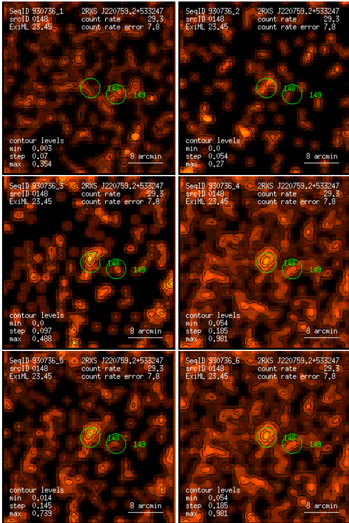
Figure 148: RASS 930736: detection 0148: band rate images, Gaussian filter: (1) PSPC channels 11 – 41, (2) 52 – 90, (3) 91 – 201, (4) 11 – 235, (5) 52 – 201, (6) 11 – 201. Broad band rates in counts/ks. Band rate contour levels in counts/ks/arcmin 2 .
