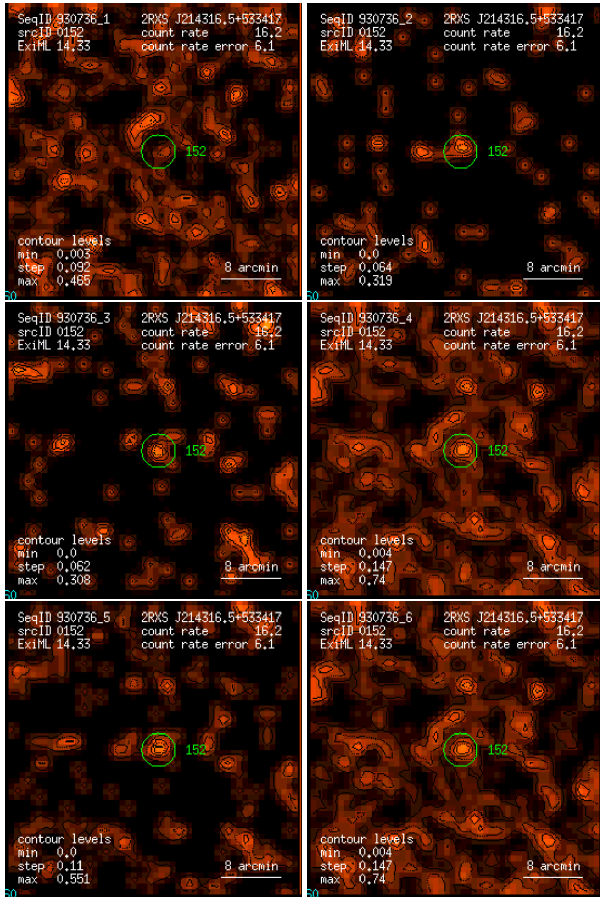
Figure 152: RASS 930736: detection 0152: band rate images, Gaussian filter: (1) PSPC channels 11 – 41, (2) 52 – 90, (3) 91 – 201, (4) 11 – 235, (5) 52 – 201, (6) 11 – 201. Broad band rates in counts/ks. Band rate contour levels in counts/ks/arcmin 2 .
