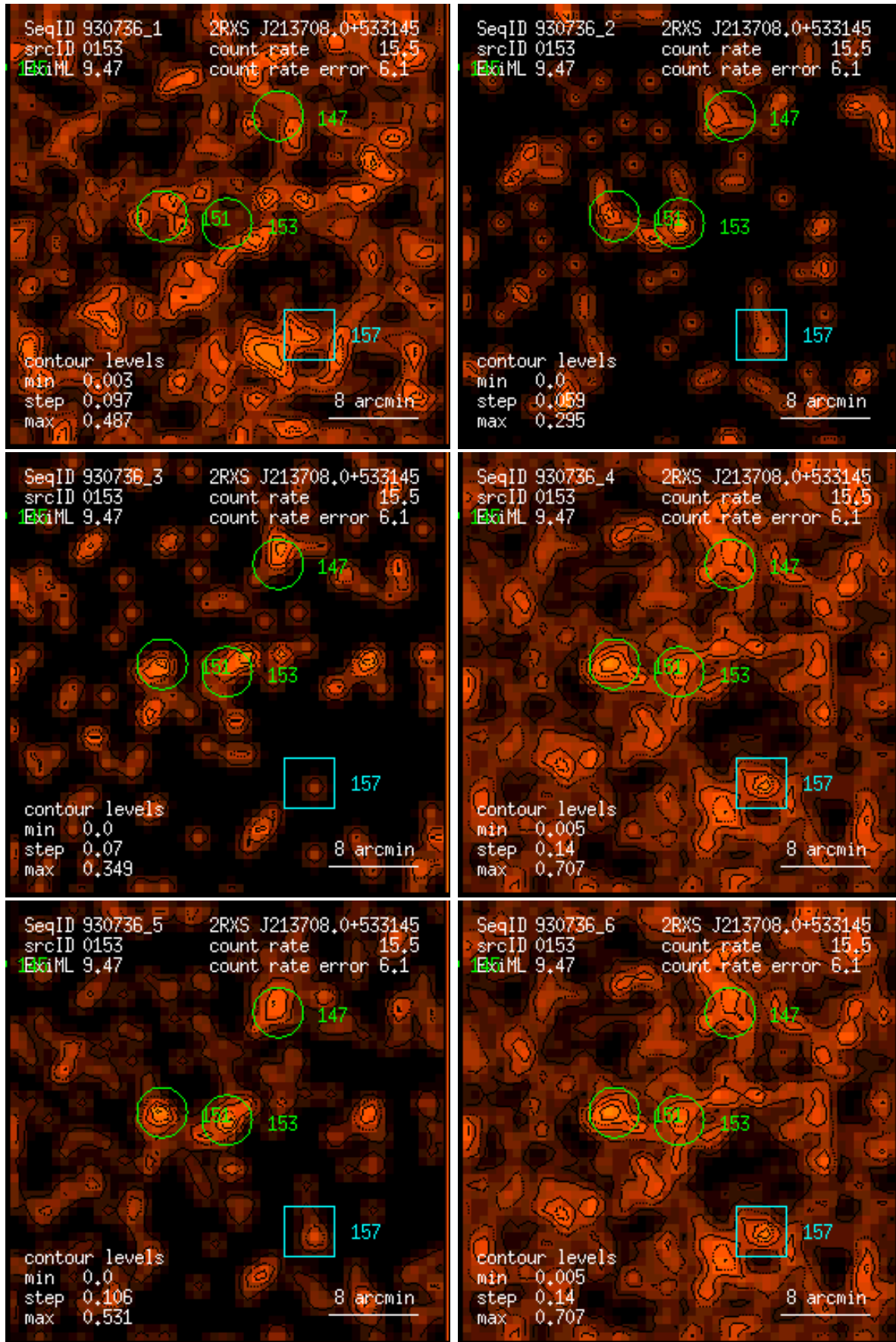
Figure 153: RASS 930736: detection 0153: band rate images, Gaussian filter: (1) PSPC channels 11 – 41, (2) 52 – 90, (3) 91 – 201, (4) 11 – 235, (5) 52 – 201, (6) 11 – 201. Broad band rates in counts/ks. Band rate contour levels in counts/ks/arcmin 2 .
