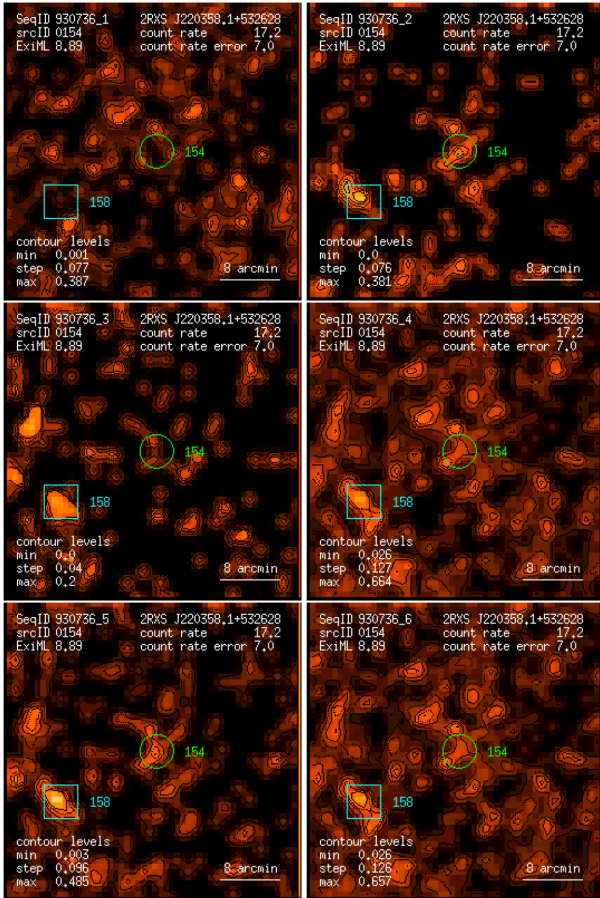
Figure 154: RASS 930736: detection 0154: band rate images, Gaussian filter: (1) PSPC channels 11 – 41, (2) 52 – 90, (3) 91 – 201, (4) 11 – 235, (5) 52 – 201, (6) 11 – 201. Broad band rates in counts/ks. Band rate contour levels in counts/ks/arcmin 2 .
