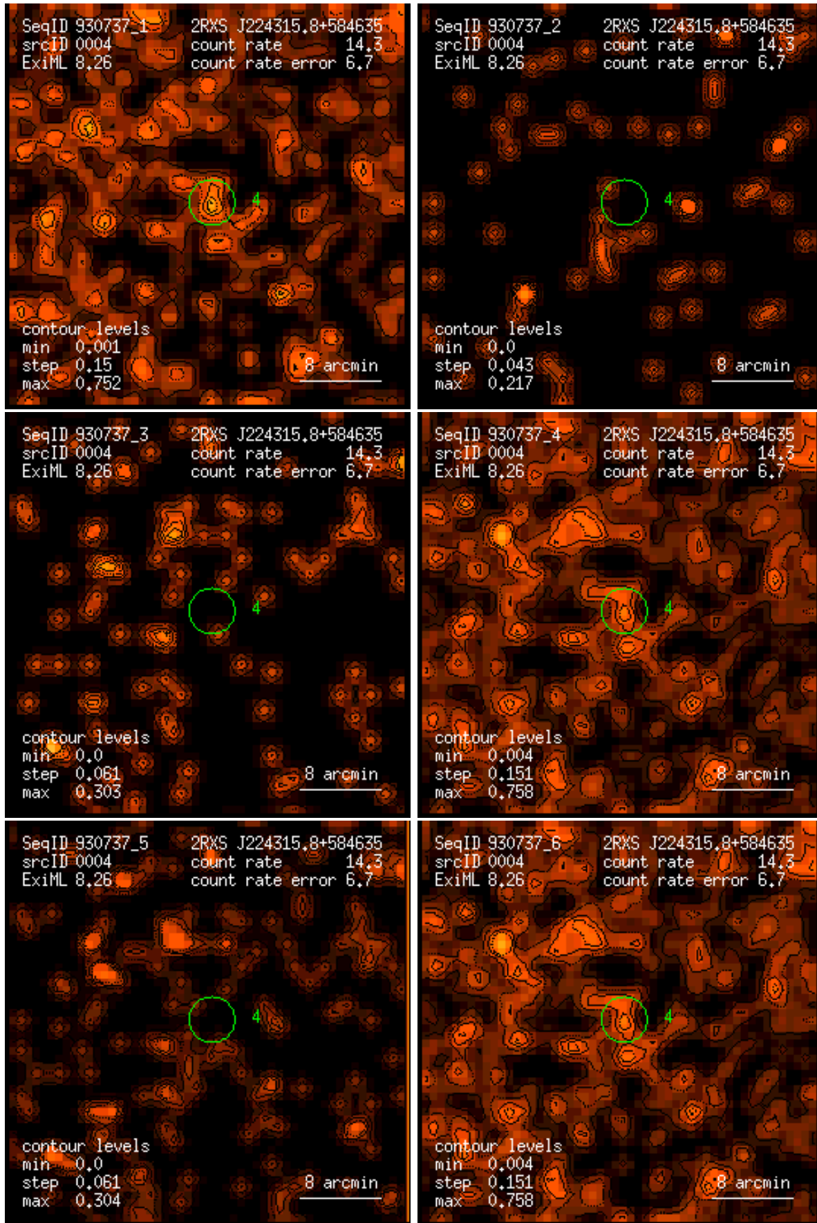
Figure 4: RASS 930737: detection 0004: band rate images, Gaussian filter: (1) PSPC channels 11 – 41, (2) 52 – 90, (3) 91 – 201, (4) 11 – 235, (5) 52 – 201, (6) 11 – 201. Broad band rates in counts/ks. Band rate contour levels in counts/ks/arcmin 2 .
