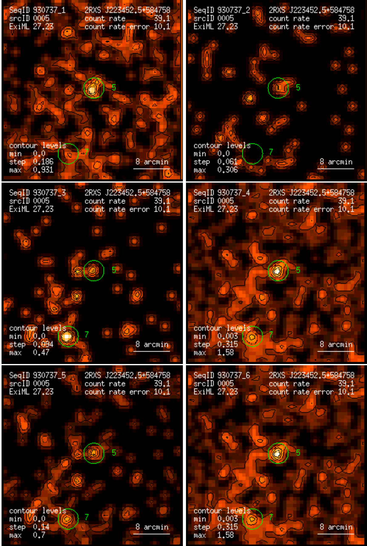
Figure 5: RASS 930737: detection 0005: band rate images, Gaussian filter: (1) PSPC channels 11 – 41, (2) 52 – 90, (3) 91 – 201, (4) 11 – 235, (5) 52 – 201, (6) 11 – 201. Broad band rates in counts/ks. Band rate contour levels in counts/ks/arcmin 2 .
