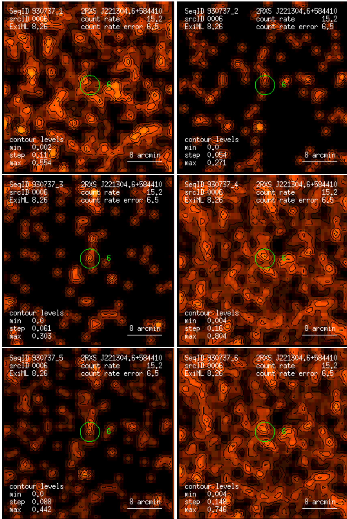
Figure 6: RASS 930737: detection 0006: band rate images, Gaussian filter: (1) PSPC channels 11 – 41, (2) 52 – 90, (3) 91 – 201, (4) 11 – 235, (5) 52 – 201, (6) 11 – 201. Broad band rates in counts/ks. Band rate contour levels in counts/ks/arcmin 2 .
