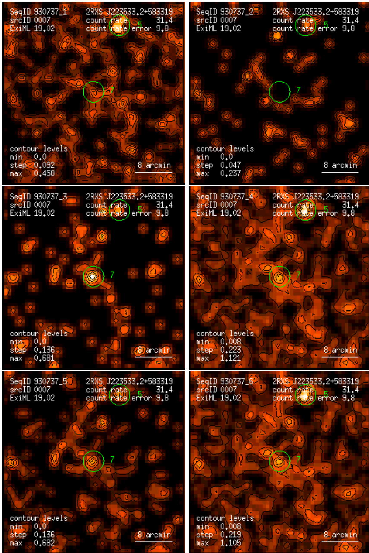
Figure 7: RASS 930737: detection 0007: band rate images, Gaussian filter: (1) PSPC channels 11 – 41, (2) 52 – 90, (3) 91 – 201, (4) 11 – 235, (5) 52 – 201, (6) 11 – 201. Broad band rates in counts/ks. Band rate contour levels in counts/ks/arcmin 2 .
