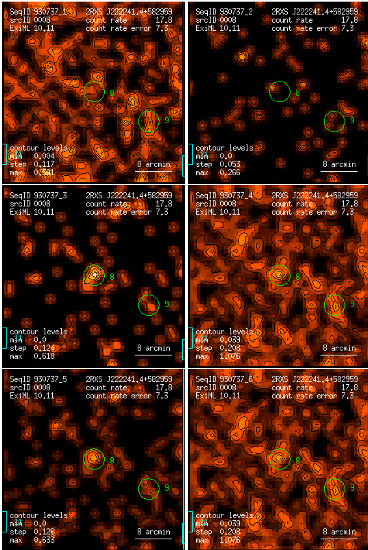
Figure 8: RASS 930737: detection 0008: band rate images, Gaussian filter: (1) PSPC channels 11 – 41, (2) 52 – 90, (3) 91 – 201, (4) 11 – 235, (5) 52 – 201, (6) 11 – 201. Broad band rates in counts/ks. Band rate contour levels in counts/ks/arcmin 2 .
