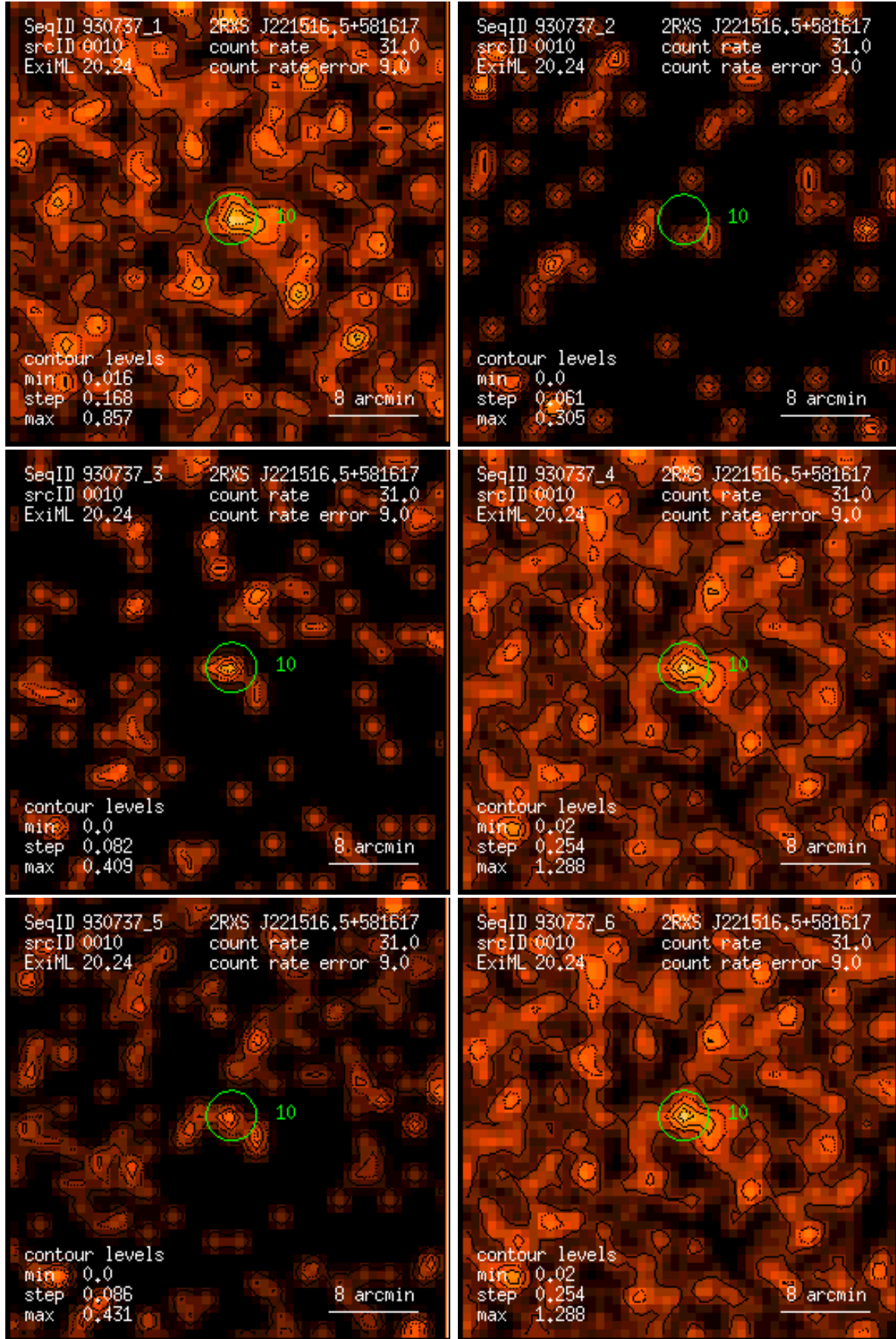
Figure 10: RASS 930737: detection 0010: band rate images, Gaussian filter: (1) PSPC channels 11 – 41, (2) 52 – 90, (3) 91 – 201, (4) 11 – 235, (5) 52 – 201, (6) 11 – 201. Broad band rates in counts/ks. Band rate contour levels in counts/ks/arcmin 2 .
