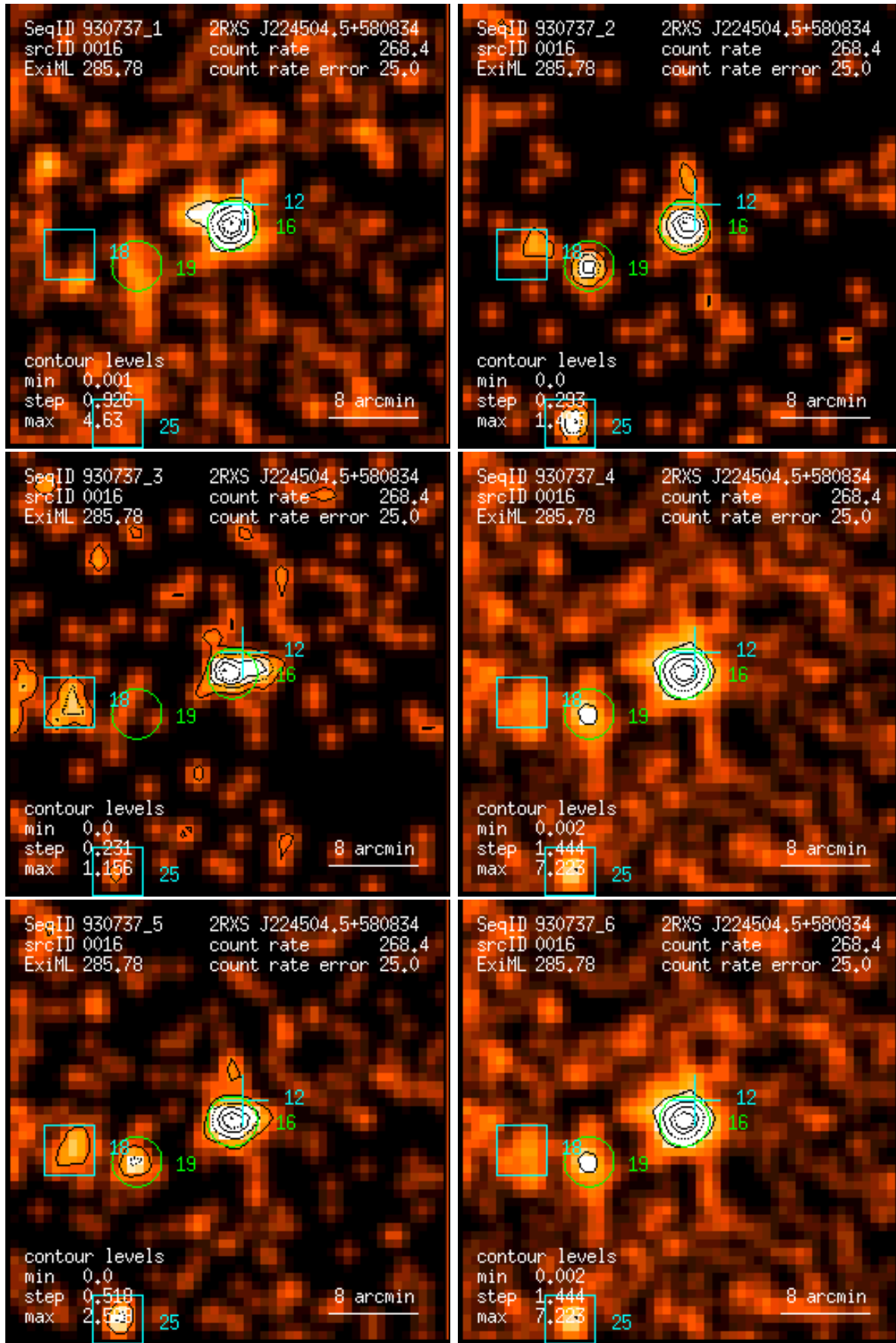
Figure 16: RASS 930737: detection 0016: band rate images, Gaussian filter: (1) PSPC channels 11 – 41, (2) 52 – 90, (3) 91 – 201, (4) 11 – 235, (5) 52 – 201, (6) 11 – 201. Broad band rates in counts/ks. Band rate contour levels in counts/ks/arcmin 2 .
