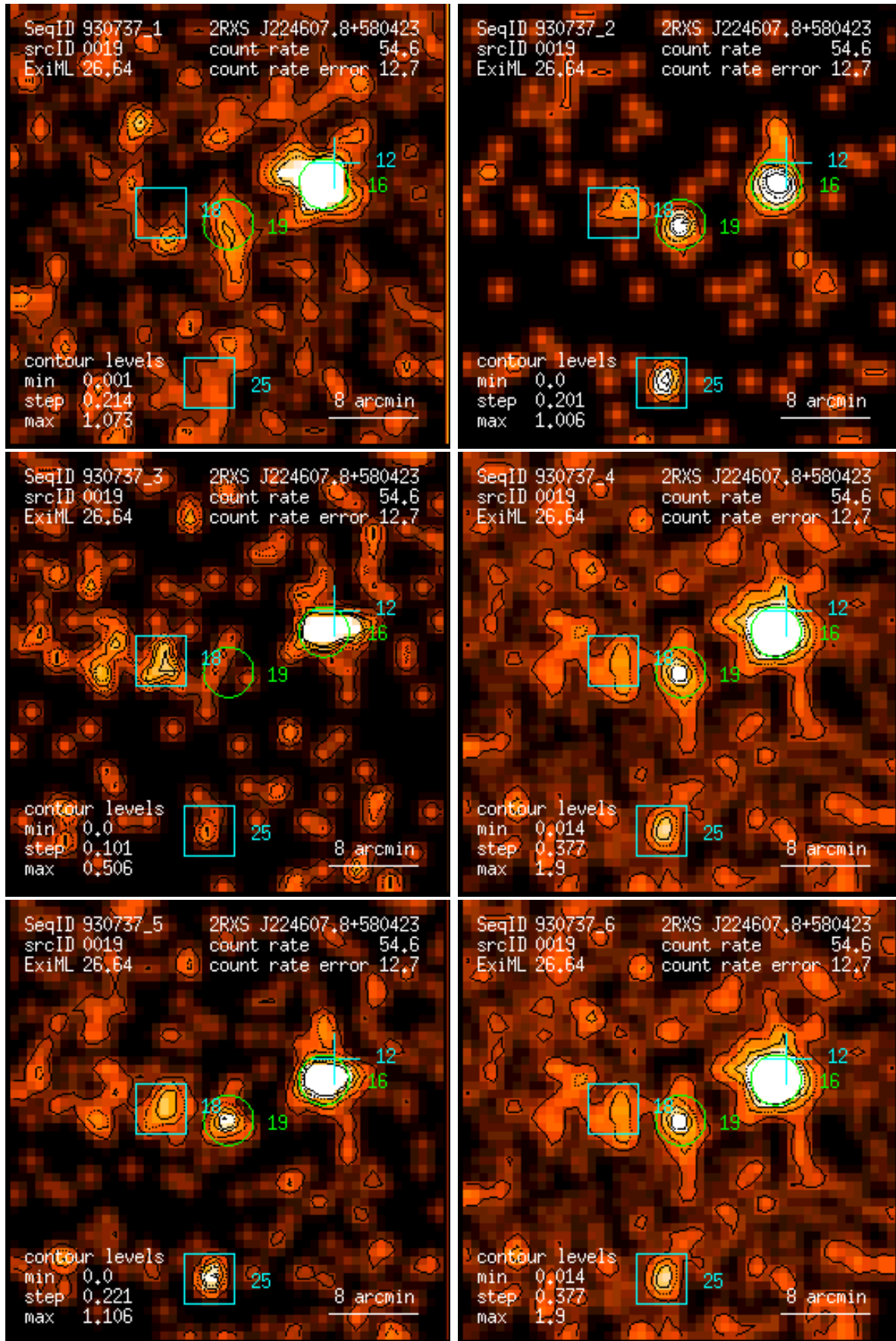
Figure 19: RASS 930737: detection 0019: band rate images, Gaussian filter: (1) PSPC channels 11 – 41, (2) 52 – 90, (3) 91 – 201, (4) 11 – 235, (5) 52 – 201, (6) 11 – 201. Broad band rates in counts/ks. Band rate contour levels in counts/ks/arcmin 2 .
