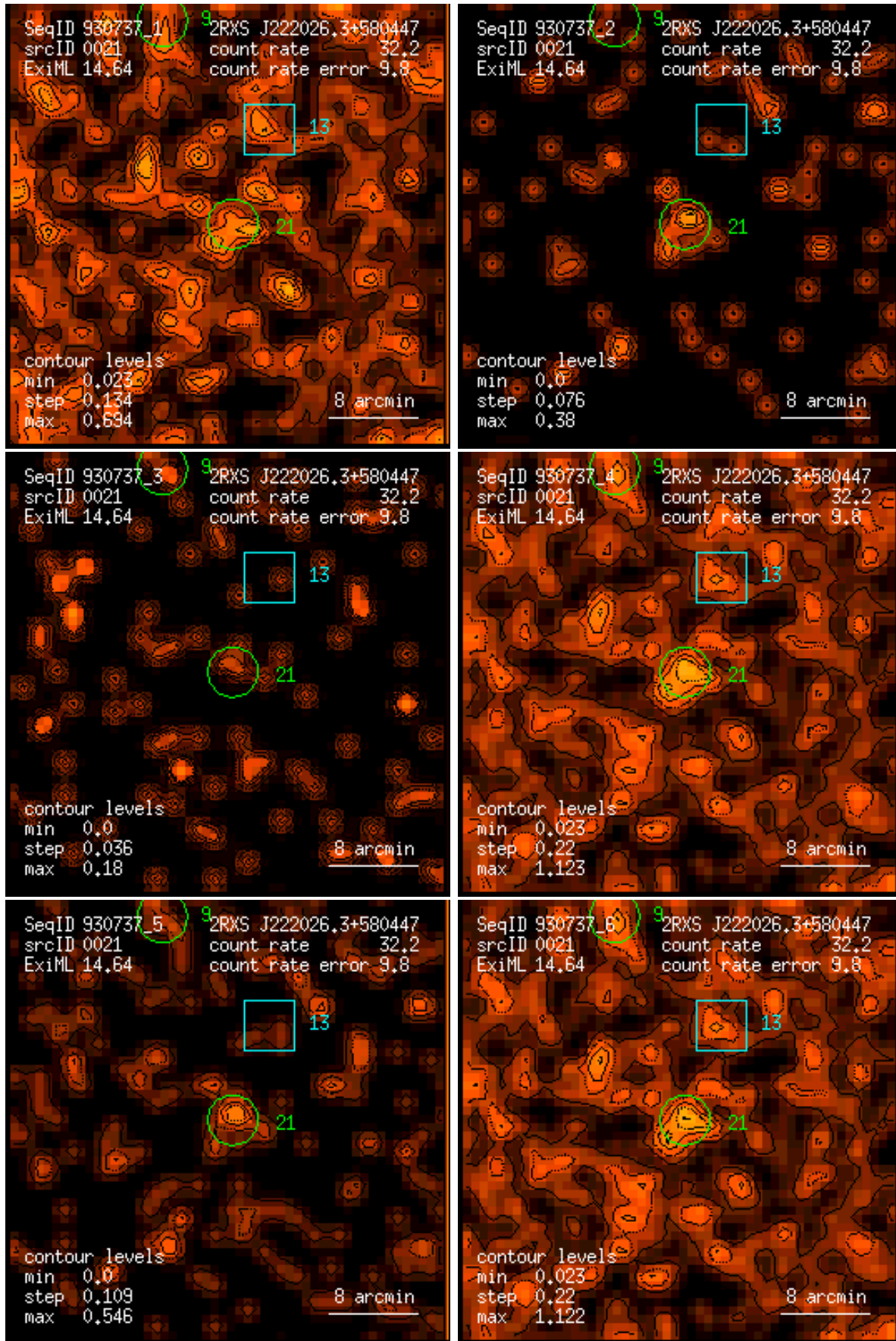
Figure 21: RASS 930737: detection 0021: band rate images, Gaussian filter: (1) PSPC channels 11 – 41, (2) 52 – 90, (3) 91 – 201, (4) 11 – 235, (5) 52 – 201, (6) 11 – 201. Broad band rates in counts/ks. Band rate contour levels in counts/ks/arcmin 2 .
