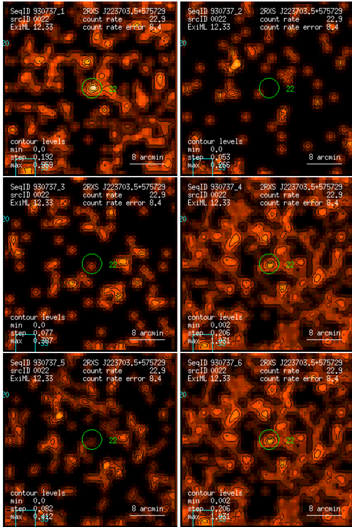
Figure 22: RASS 930737: detection 0022: band rate images, Gaussian filter: (1) PSPC channels 11 – 41, (2) 52 – 90, (3) 91 – 201, (4) 11 – 235, (5) 52 – 201, (6) 11 – 201. Broad band rates in counts/ks. Band rate contour levels in counts/ks/arcmin 2 .
