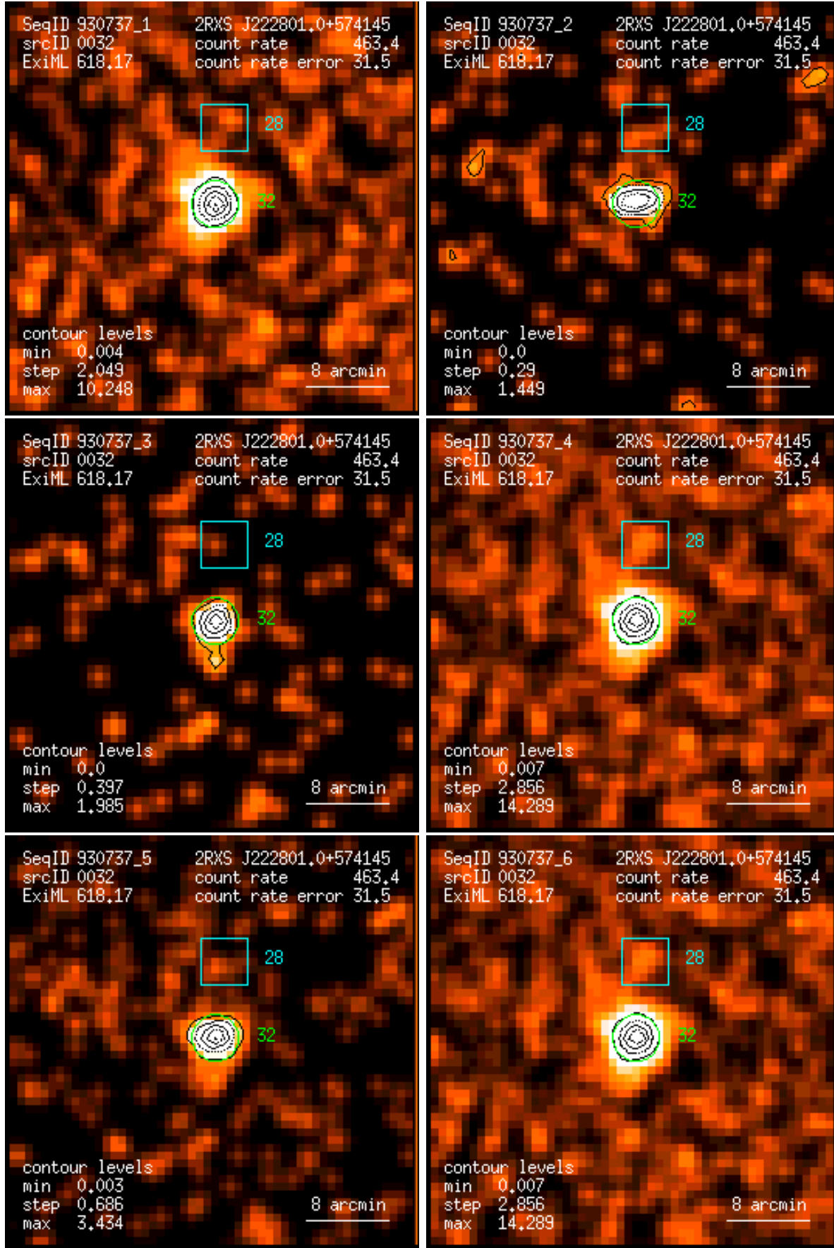
Figure 32: RASS 930737: detection 0032: band rate images, Gaussian filter: (1) PSPC channels 11 – 41, (2) 52 – 90, (3) 91 – 201, (4) 11 – 235, (5) 52 – 201, (6) 11 – 201. Broad band rates in counts/ks. Band rate contour levels in counts/ks/arcmin 2 .
