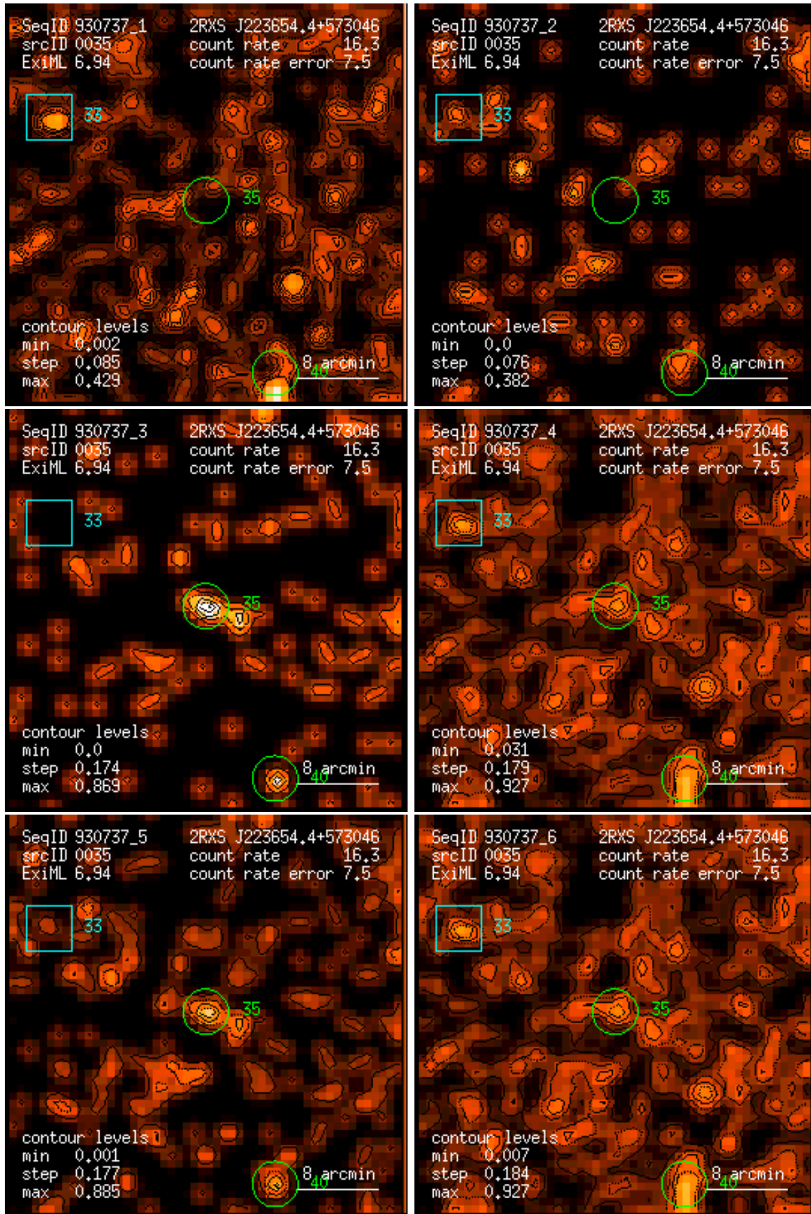
Figure 35: RASS 930737: detection 0035: band rate images, Gaussian filter: (1) PSPC channels 11 – 41, (2) 52 – 90, (3) 91 – 201, (4) 11 – 235, (5) 52 – 201, (6) 11 – 201. Broad band rates in counts/ks. Band rate contour levels in counts/ks/arcmin 2 .
