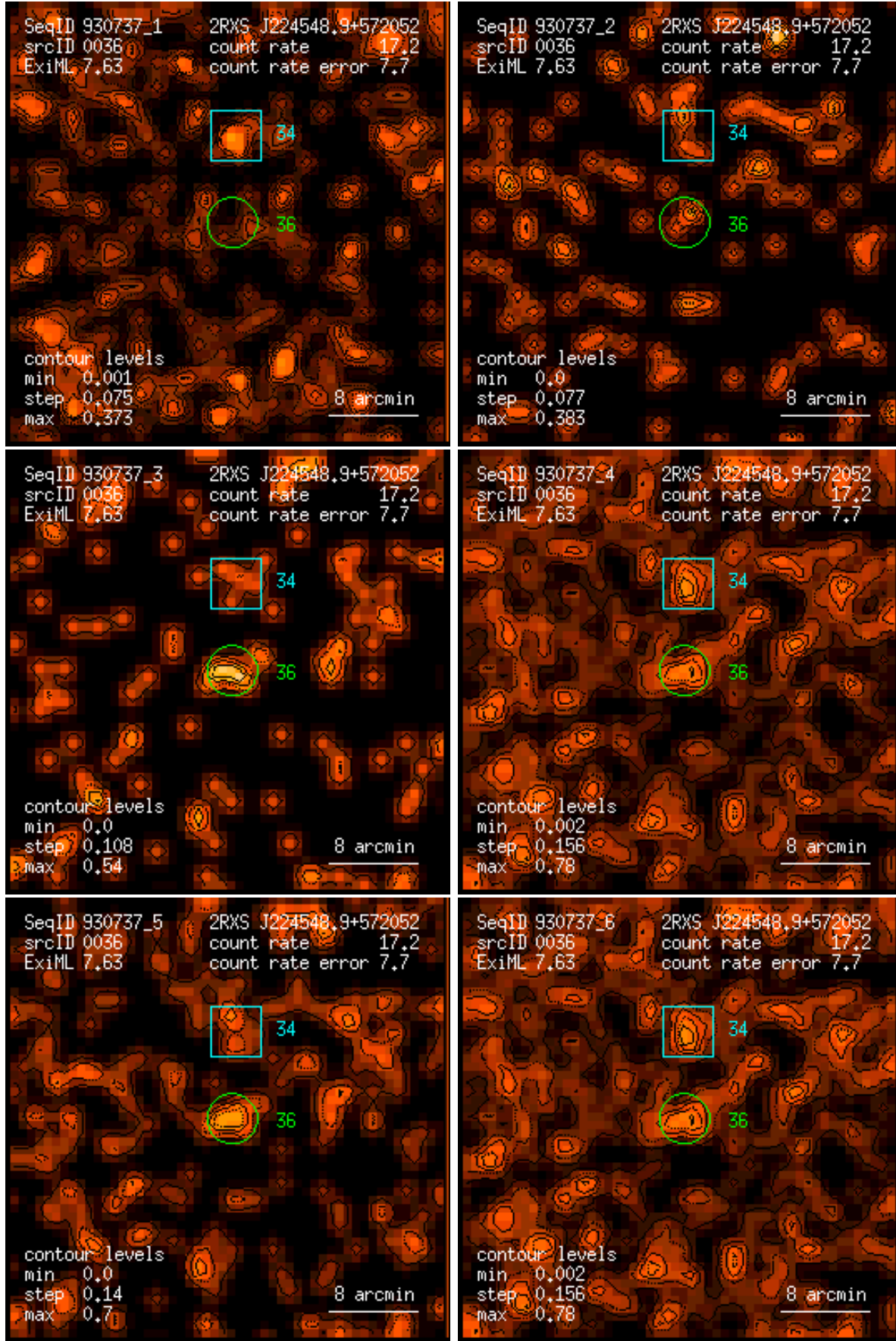
Figure 36: RASS 930737: detection 0036: band rate images, Gaussian filter: (1) PSPC channels 11 – 41, (2) 52 – 90, (3) 91 – 201, (4) 11 – 235, (5) 52 – 201, (6) 11 – 201. Broad band rates in counts/ks. Band rate contour levels in counts/ks/arcmin 2 .
