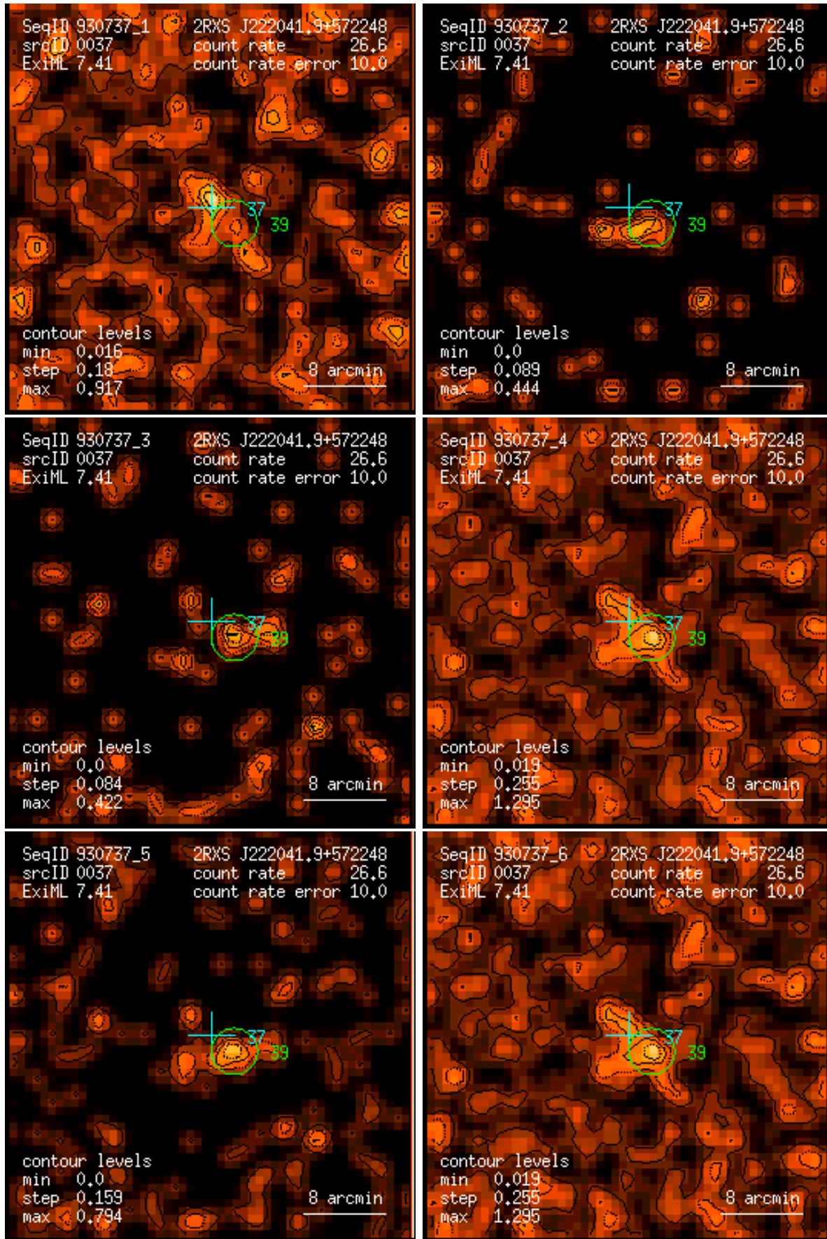
Figure 37: RASS 930737: detection 0037: band rate images, Gaussian filter: (1) PSPC channels 11 – 41, (2) 52 – 90, (3) 91 – 201, (4) 11 – 235, (5) 52 – 201, (6) 11 – 201. Broad band rates in counts/ks. Band rate contour levels in counts/ks/arcmin 2 .
