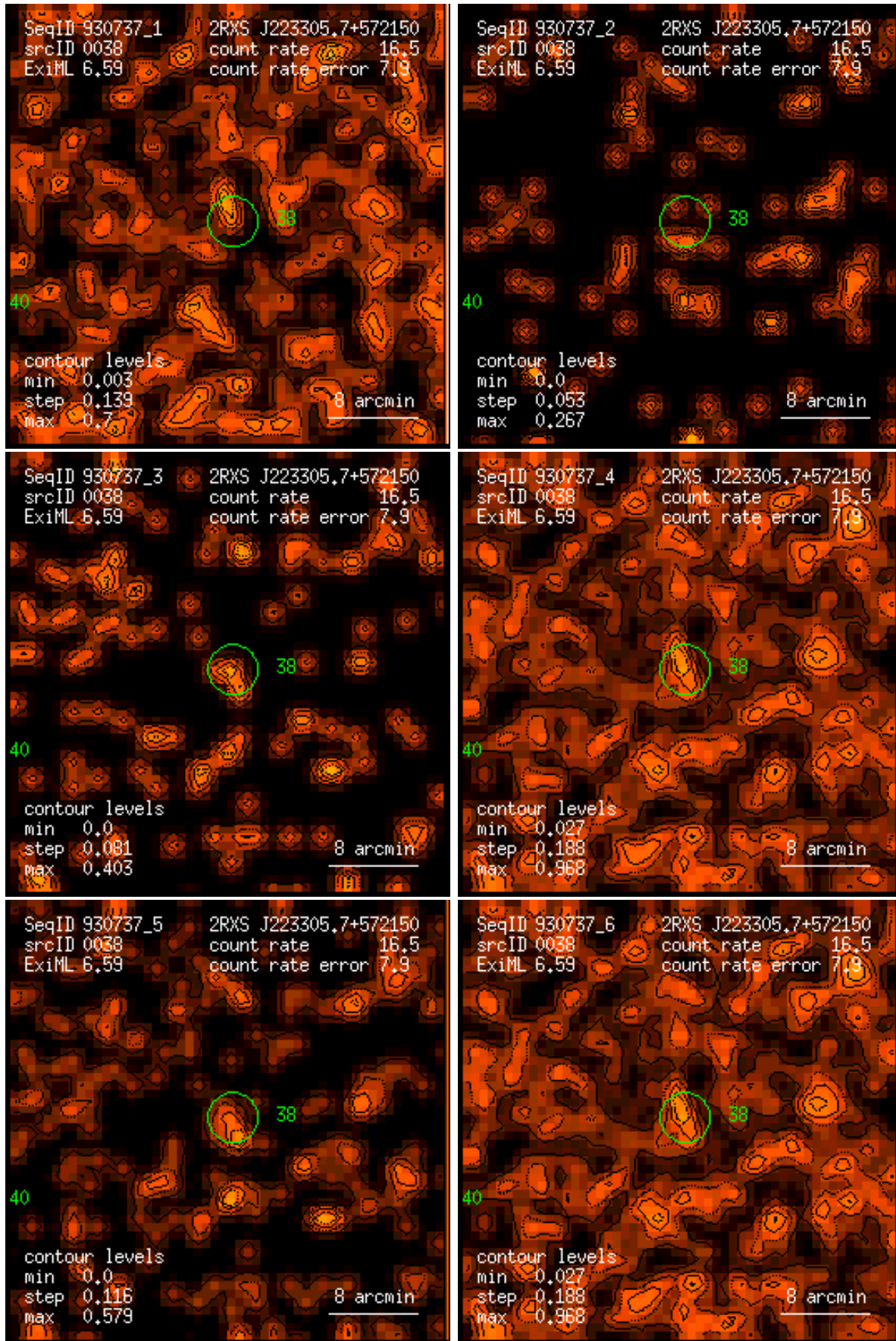
Figure 38: RASS 930737: detection 0038: band rate images, Gaussian filter: (1) PSPC channels 11 – 41, (2) 52 – 90, (3) 91 – 201, (4) 11 – 235, (5) 52 – 201, (6) 11 – 201. Broad band rates in counts/ks. Band rate contour levels in counts/ks/arcmin 2 .
