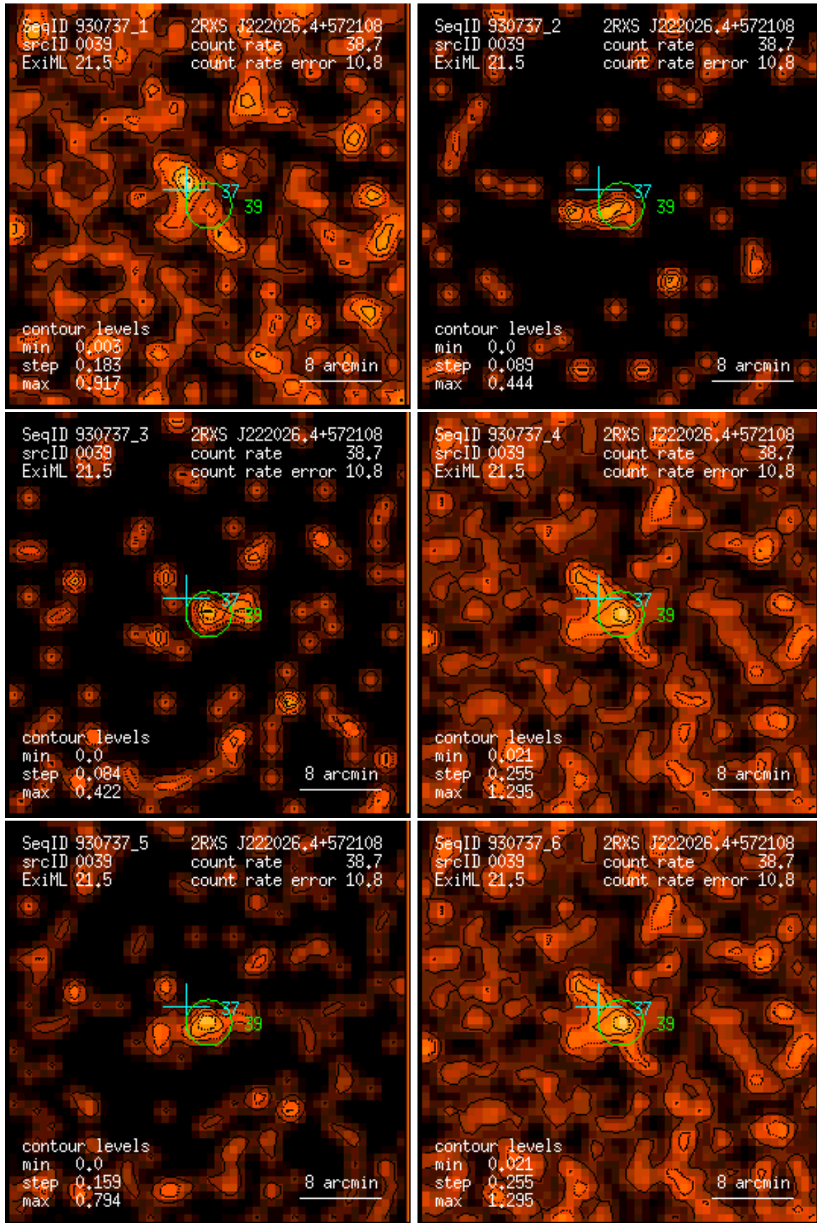
Figure 39: RASS 930737: detection 0039: band rate images, Gaussian filter: (1) PSPC channels 11 – 41, (2) 52 – 90, (3) 91 – 201, (4) 11 – 235, (5) 52 – 201, (6) 11 – 201. Broad band rates in counts/ks. Band rate contour levels in counts/ks/arcmin 2 .
