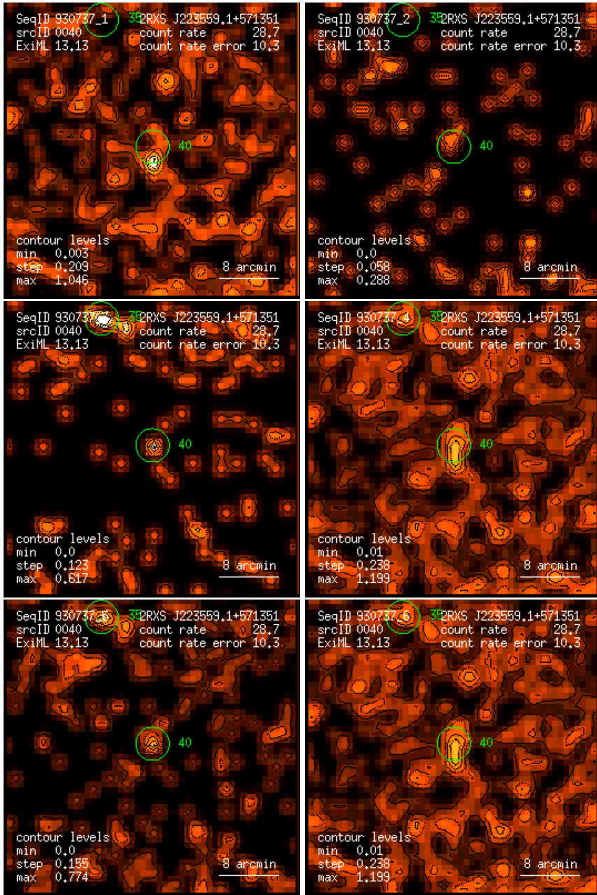
Figure 40: RASS 930737: detection 0040: band rate images, Gaussian filter: (1) PSPC channels 11 – 41, (2) 52 – 90, (3) 91 – 201, (4) 11 – 235, (5) 52 – 201, (6) 11 – 201. Broad band rates in counts/ks. Band rate contour levels in counts/ks/arcmin 2 .
