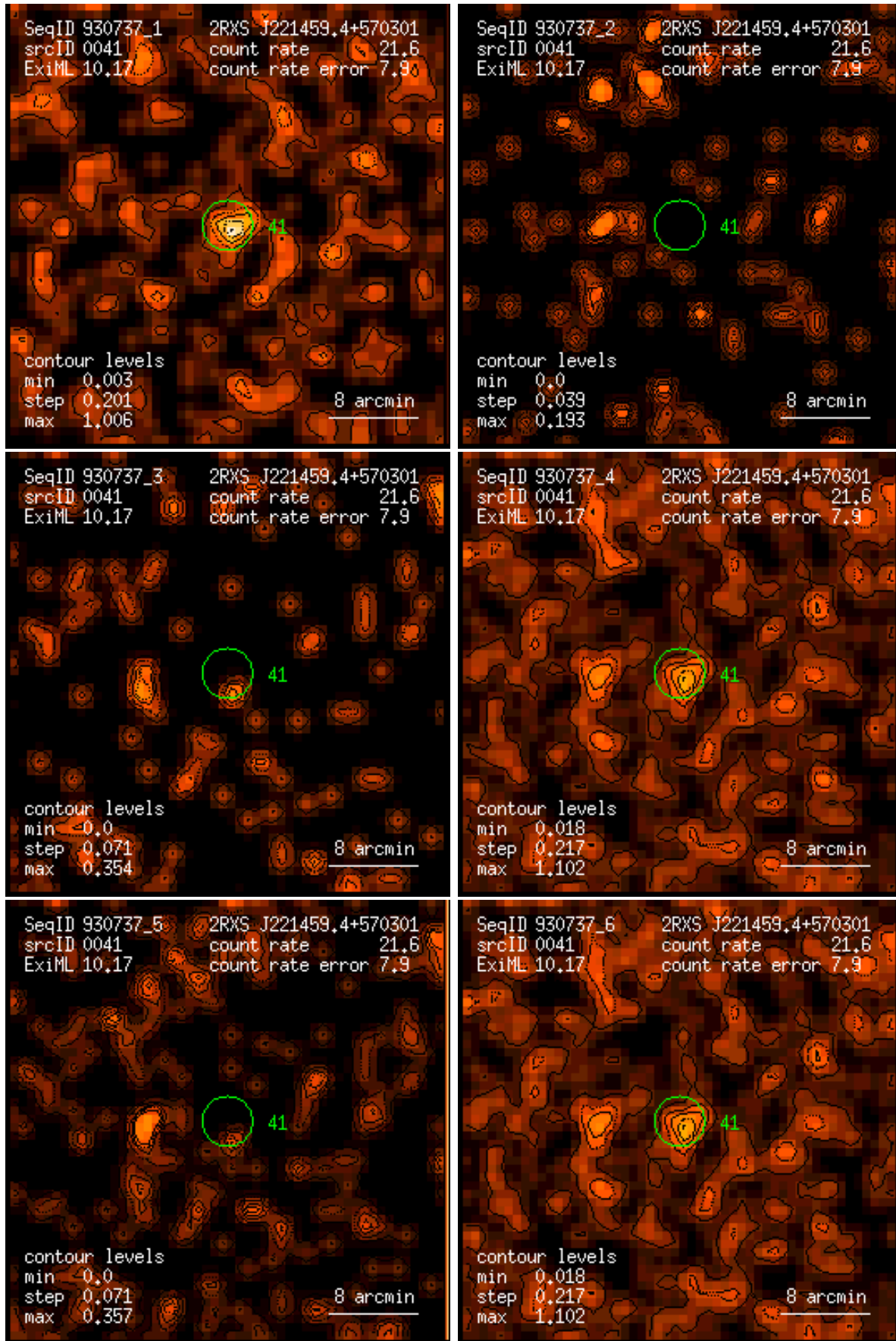
Figure 41: RASS 930737: detection 0041: band rate images, Gaussian filter: (1) PSPC channels 11 – 41, (2) 52 – 90, (3) 91 – 201, (4) 11 – 235, (5) 52 – 201, (6) 11 – 201. Broad band rates in counts/ks. Band rate contour levels in counts/ks/arcmin 2 .
