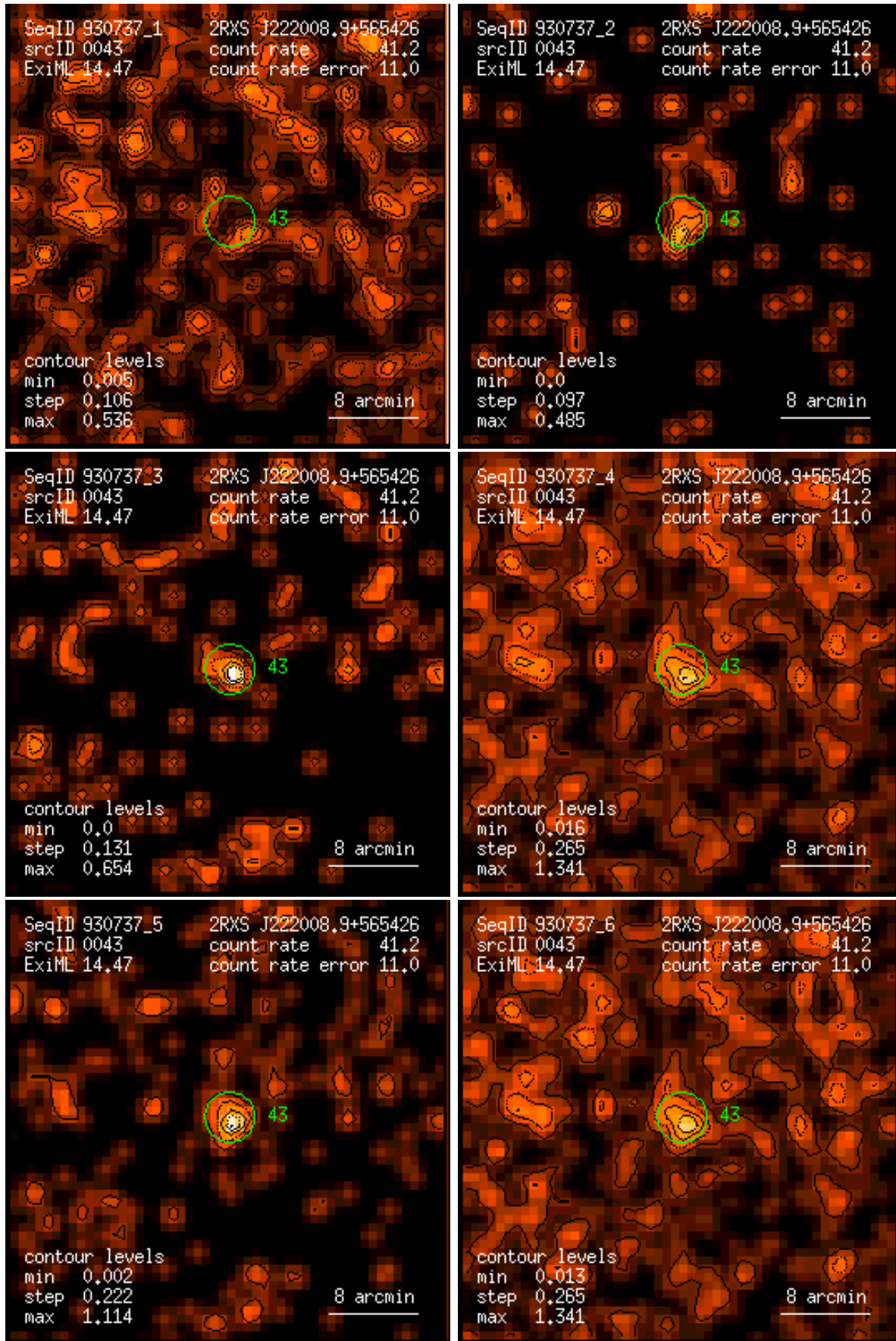
Figure 43: RASS 930737: detection 0043: band rate images, Gaussian filter: (1) PSPC channels 11 – 41, (2) 52 – 90, (3) 91 – 201, (4) 11 – 235, (5) 52 – 201, (6) 11 – 201. Broad band rates in counts/ks. Band rate contour levels in counts/ks/arcmin 2 .
