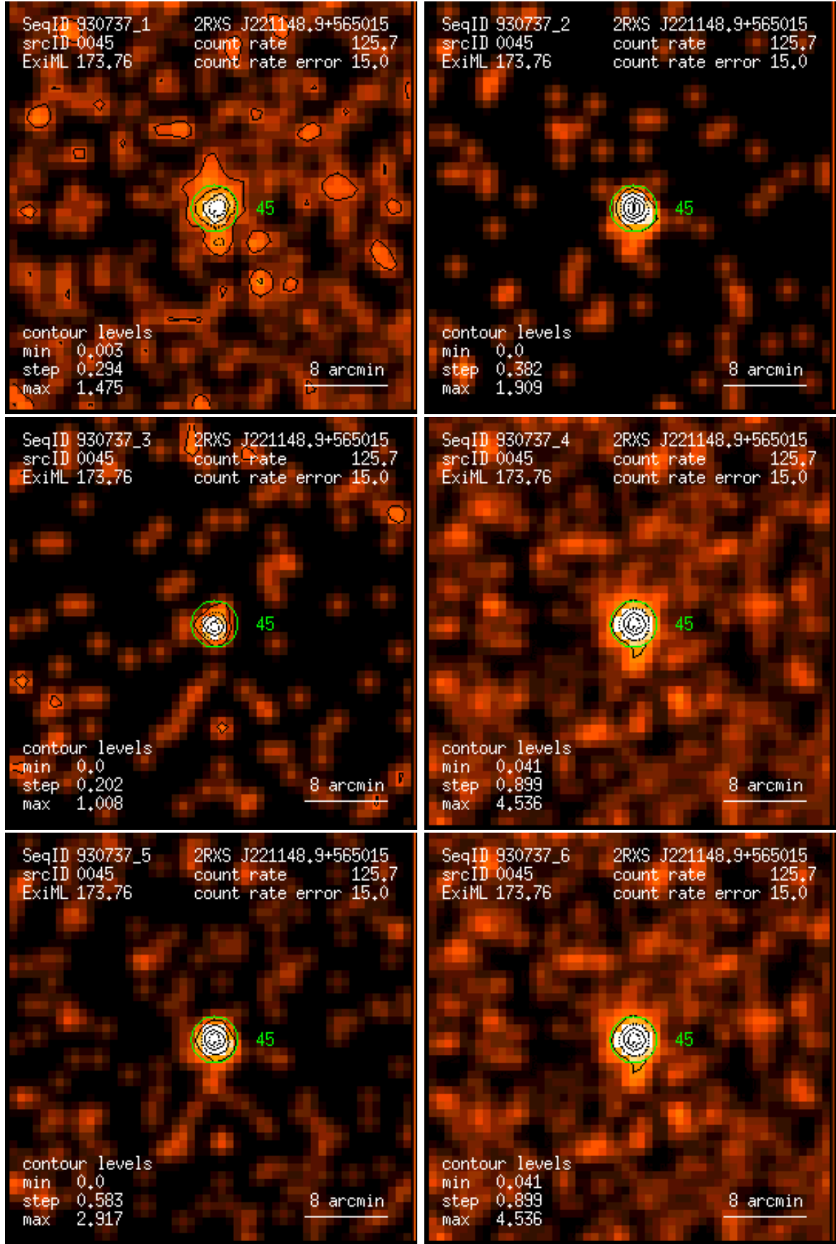
Figure 45: RASS 930737: detection 0045: band rate images, Gaussian filter: (1) PSPC channels 11 – 41, (2) 52 – 90, (3) 91 – 201, (4) 11 – 235, (5) 52 – 201, (6) 11 – 201. Broad band rates in counts/ks. Band rate contour levels in counts/ks/arcmin 2 .
