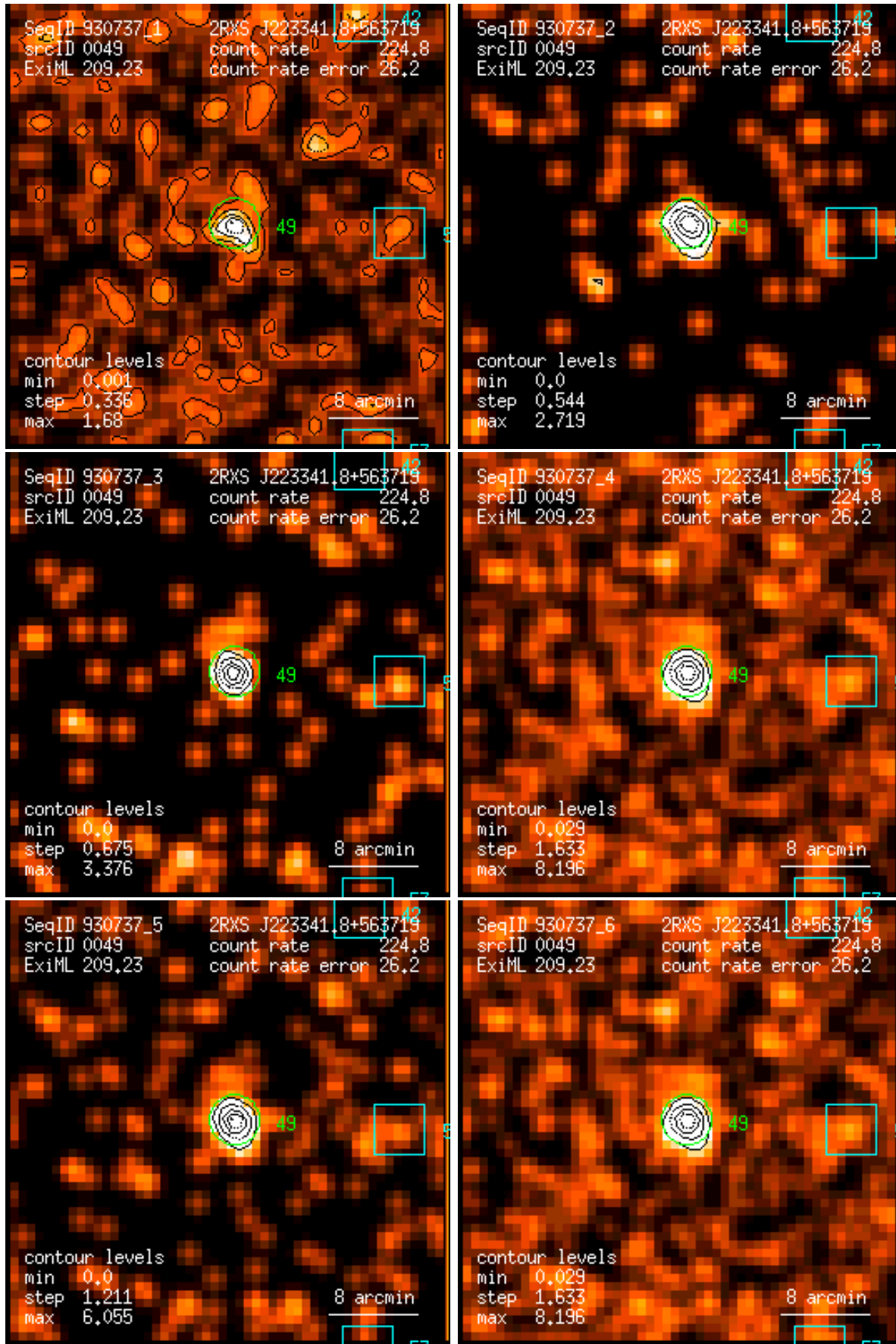
Figure 49: RASS 930737: detection 0049: band rate images, Gaussian filter: (1) PSPC channels 11 – 41, (2) 52 – 90, (3) 91 – 201, (4) 11 – 235, (5) 52 – 201, (6) 11 – 201. Broad band rates in counts/ks. Band rate contour levels in counts/ks/arcmin 2 .
