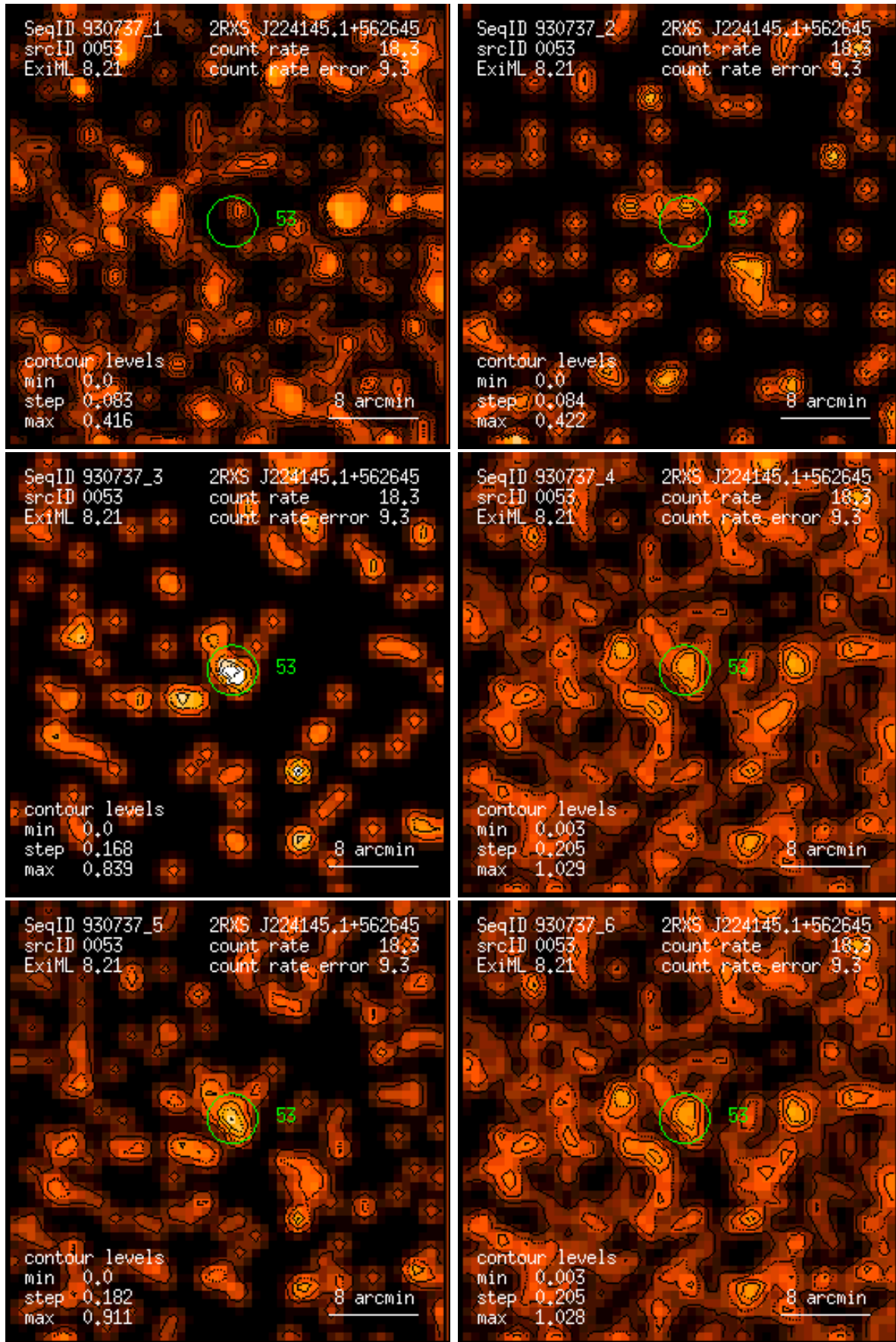
Figure 53: RASS 930737: detection 0053: band rate images, Gaussian filter: (1) PSPC channels 11 – 41, (2) 52 – 90, (3) 91 – 201, (4) 11 – 235, (5) 52 – 201, (6) 11 – 201. Broad band rates in counts/ks. Band rate contour levels in counts/ks/arcmin 2 .
