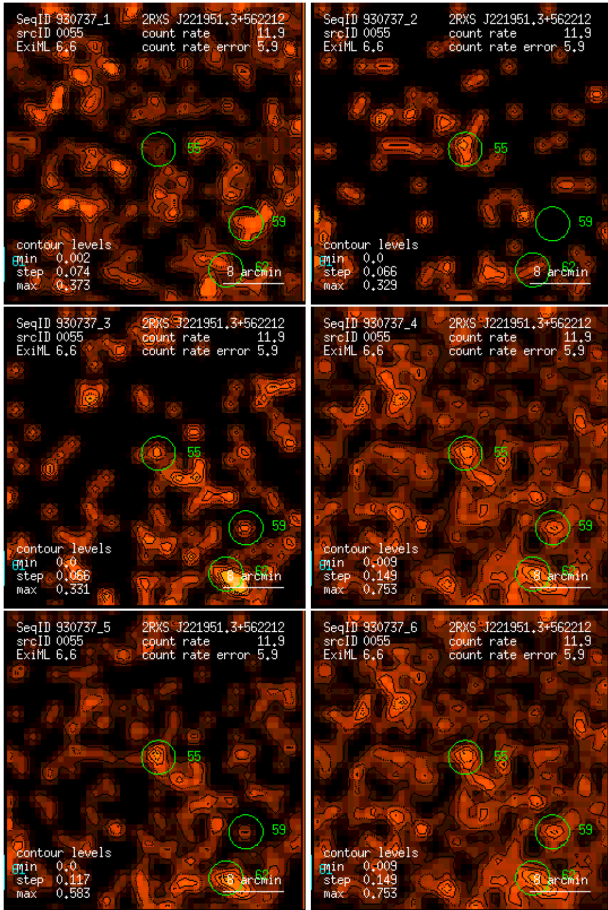
Figure 55: RASS 930737: detection 0055: band rate images, Gaussian filter: (1) PSPC channels 11 – 41, (2) 52 – 90, (3) 91 – 201, (4) 11 – 235, (5) 52 – 201, (6) 11 – 201. Broad band rates in counts/ks. Band rate contour levels in counts/ks/arcmin 2 .
