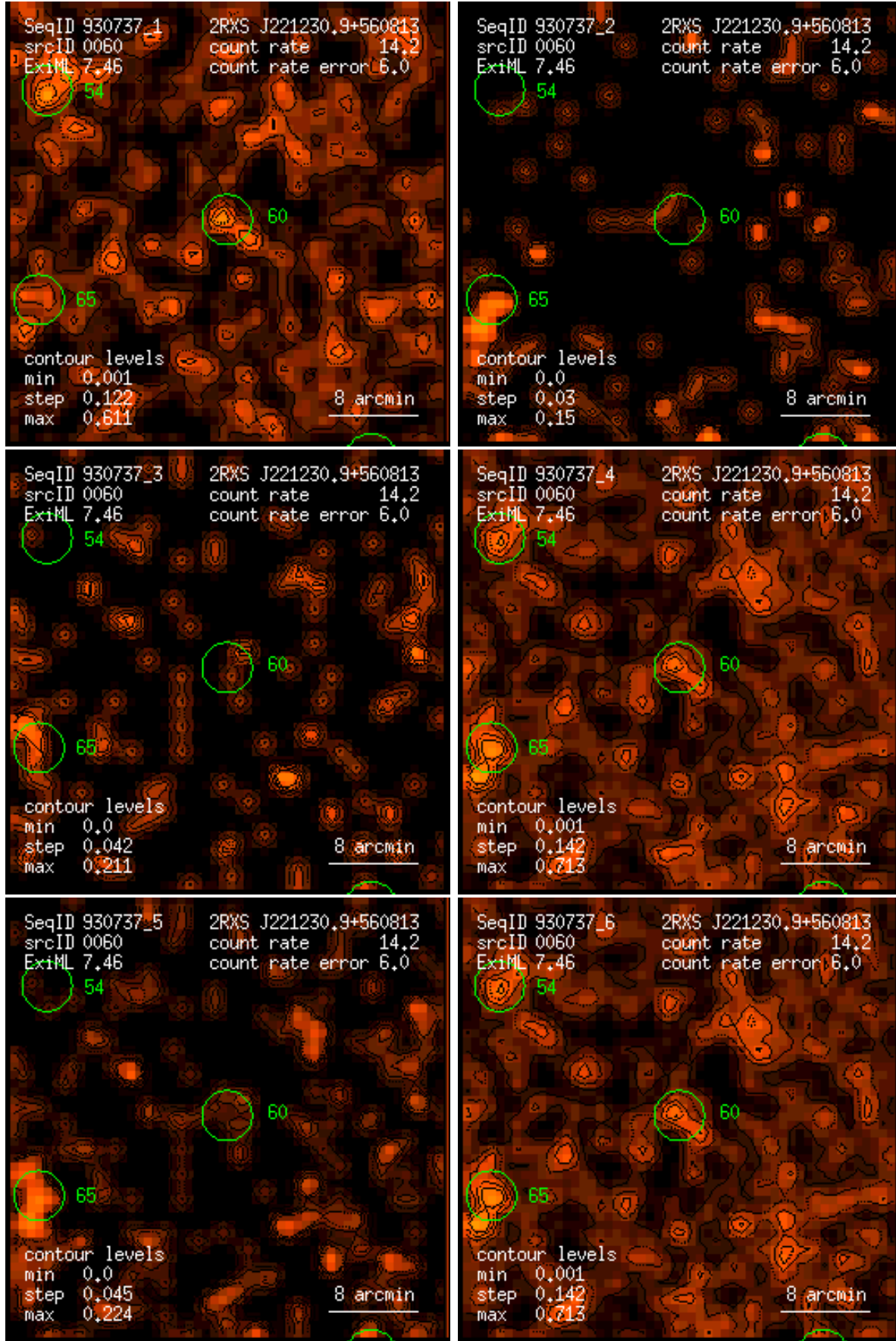
Figure 60: RASS 930737: detection 0060: band rate images, Gaussian filter: (1) PSPC channels 11 – 41, (2) 52 – 90, (3) 91 – 201, (4) 11 – 235, (5) 52 – 201, (6) 11 – 201. Broad band rates in counts/ks. Band rate contour levels in counts/ks/arcmin 2 .
