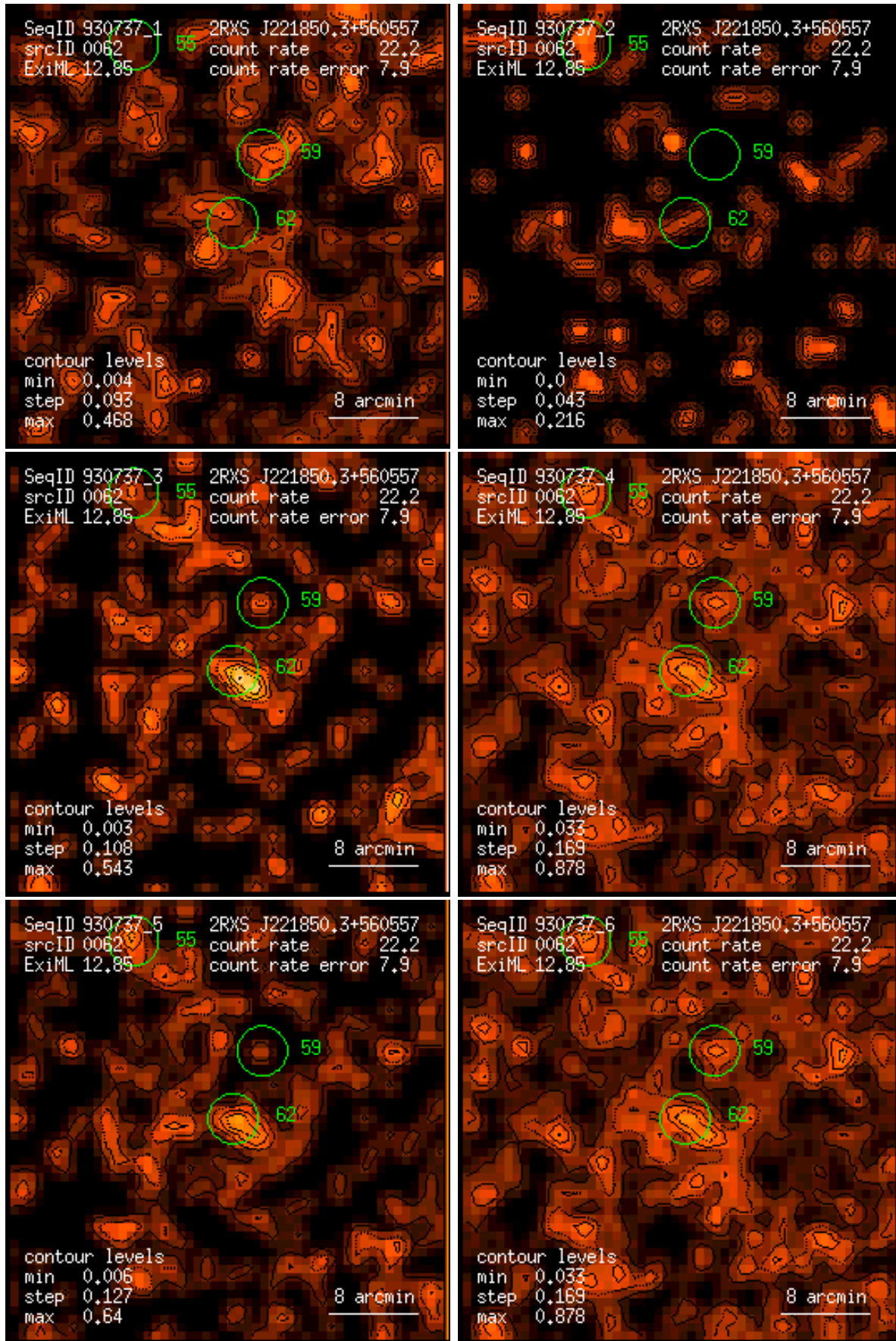
Figure 62: RASS 930737: detection 0062: band rate images, Gaussian filter: (1) PSPC channels 11 – 41, (2) 52 – 90, (3) 91 – 201, (4) 11 – 235, (5) 52 – 201, (6) 11 – 201. Broad band rates in counts/ks. Band rate contour levels in counts/ks/arcmin 2 .
