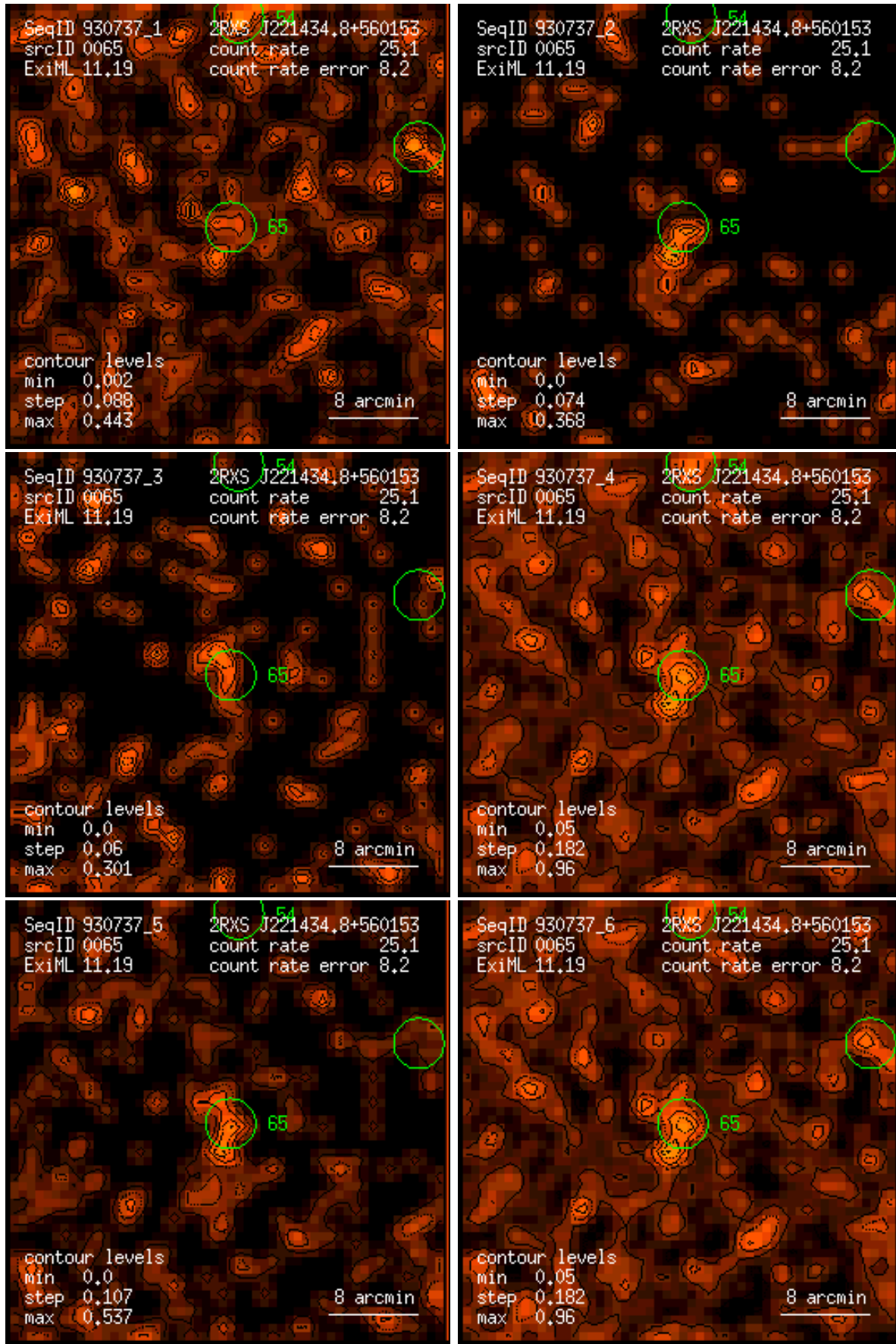
Figure 65: RASS 930737: detection 0065: band rate images, Gaussian filter: (1) PSPC channels 11 – 41, (2) 52 – 90, (3) 91 – 201, (4) 11 – 235, (5) 52 – 201, (6) 11 – 201. Broad band rates in counts/ks. Band rate contour levels in counts/ks/arcmin 2 .
