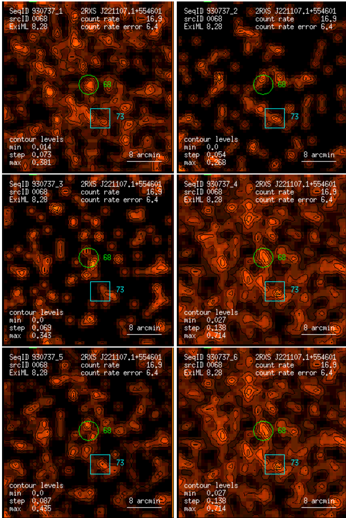
Figure 68: RASS 930737: detection 0068: band rate images, Gaussian filter: (1) PSPC channels 11 – 41, (2) 52 – 90, (3) 91 – 201, (4) 11 – 235, (5) 52 – 201, (6) 11 – 201. Broad band rates in counts/ks. Band rate contour levels in counts/ks/arcmin 2 .
