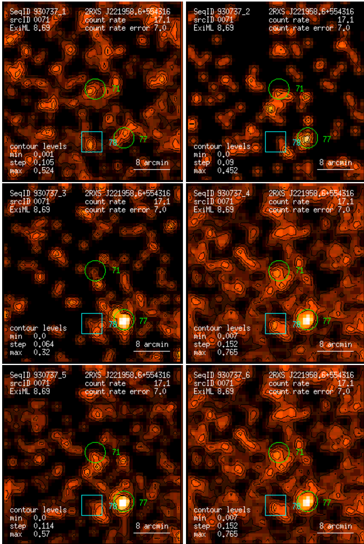
Figure 71: RASS 930737: detection 0071: band rate images, Gaussian filter: (1) PSPC channels 11 – 41, (2) 52 – 90, (3) 91 – 201, (4) 11 – 235, (5) 52 – 201, (6) 11 – 201. Broad band rates in counts/ks. Band rate contour levels in counts/ks/arcmin 2 .
