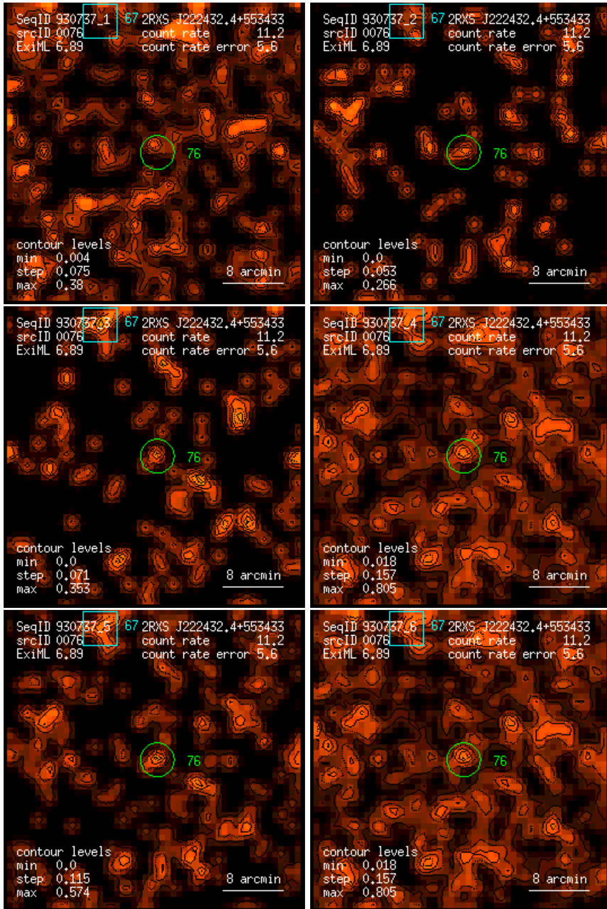
Figure 76: RASS 930737: detection 0076: band rate images, Gaussian filter: (1) PSPC channels 11 – 41, (2) 52 – 90, (3) 91 – 201, (4) 11 – 235, (5) 52 – 201, (6) 11 – 201. Broad band rates in counts/ks. Band rate contour levels in counts/ks/arcmin 2 .
