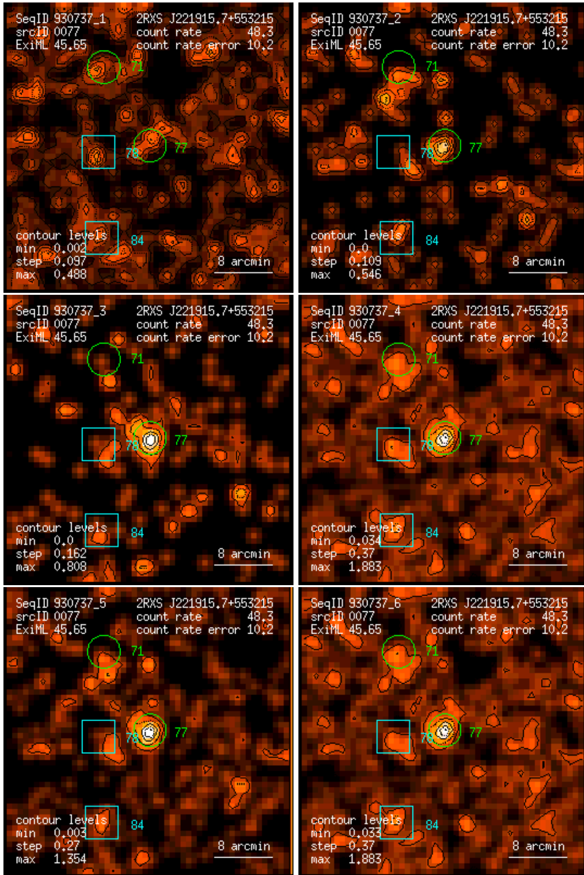
Figure 77: RASS 930737: detection 0077: band rate images, Gaussian filter: (1) PSPC channels 11 – 41, (2) 52 – 90, (3) 91 – 201, (4) 11 – 235, (5) 52 – 201, (6) 11 – 201. Broad band rates in counts/ks. Band rate contour levels in counts/ks/arcmin 2 .
