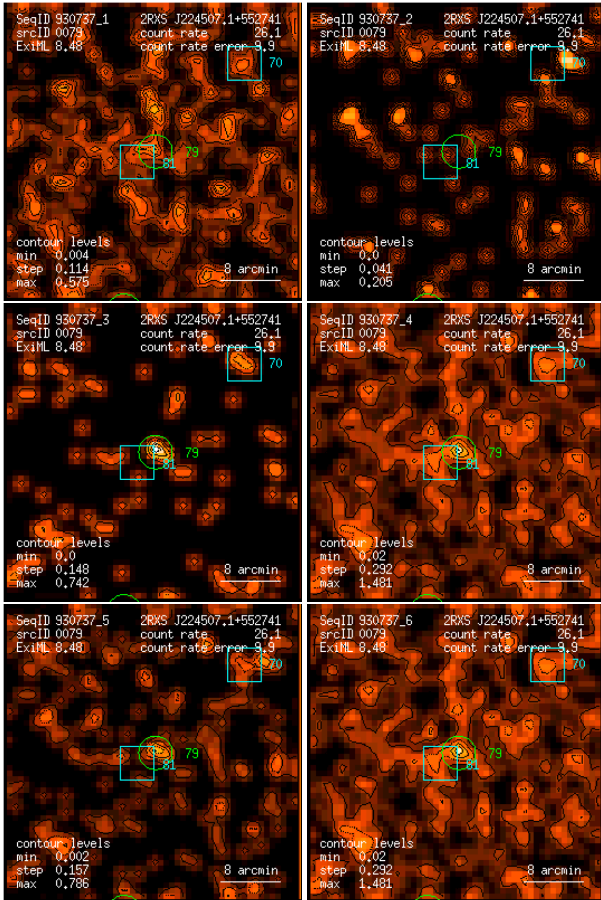
Figure 79: RASS 930737: detection 0079: band rate images, Gaussian filter: (1) PSPC channels 11 – 41, (2) 52 – 90, (3) 91 – 201, (4) 11 – 235, (5) 52 – 201, (6) 11 – 201. Broad band rates in counts/ks. Band rate contour levels in counts/ks/arcmin 2 .
